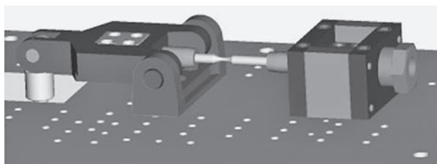
Figure 2 Load system for the bending-torsion load cycle
