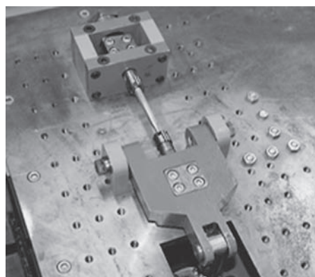
Figure 4 Multi-axial testing device
