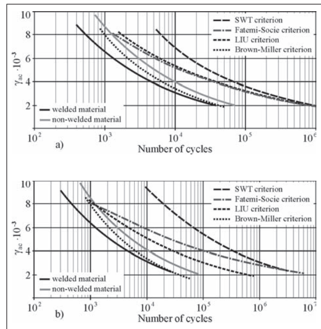
Figure 8 Comparison of the \gamma - N_f curves
