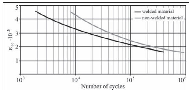
Figure 5 Manson-Coffin curves (bending)
