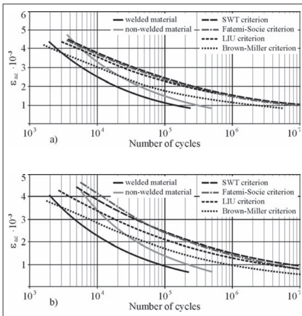
Figure 7 Comparison of the \varepsilon - N_f curves
