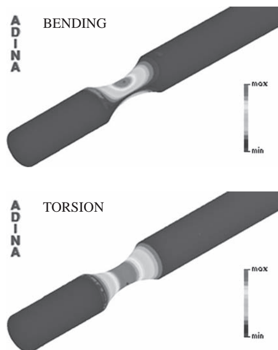
Figure 3 Distribution of equivalent von Mises stress
