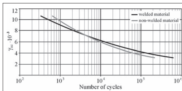
Figure 6 Manson-Coffin curves (torsion)
