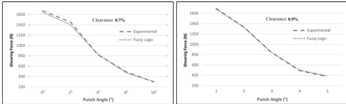
Fig. 8 Experimental results and fuzzy logic model output for clearances of 0.7%t and 0.9%t.
