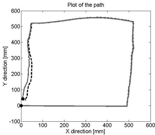
Fig. 13. Open loop test one with constant orientation
