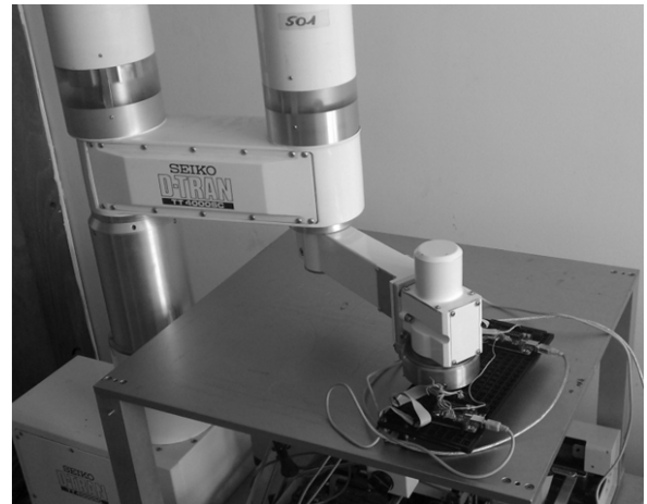
Fig. 8. SCARA measurement
