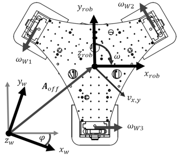
Fig. 4. Robot kinematics
