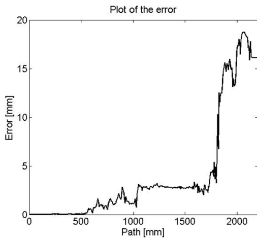
Fig. 14. Open loop test one position error
