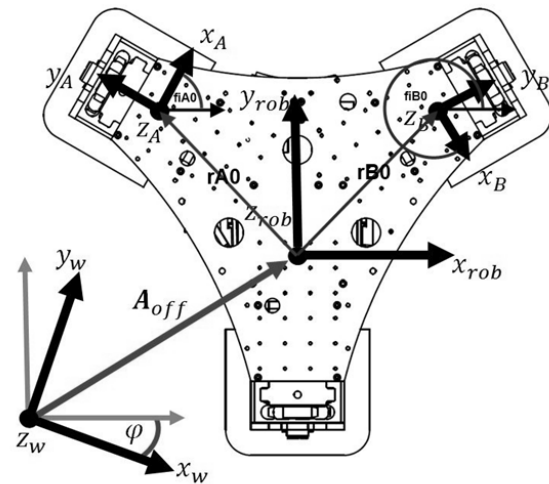
Fig. 6. Optical flow kinematics
