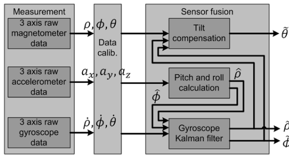
Fig. 5. 3/3/3 sensor block diagram
