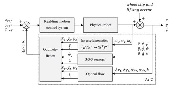
Fig. 12. System block diagram
