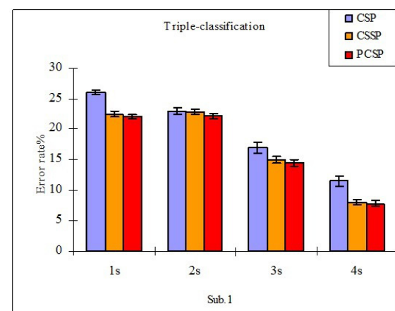
Fig. 8. Error rate and standard deviation of 10-folds cross validation for Sub.1's triple classification
