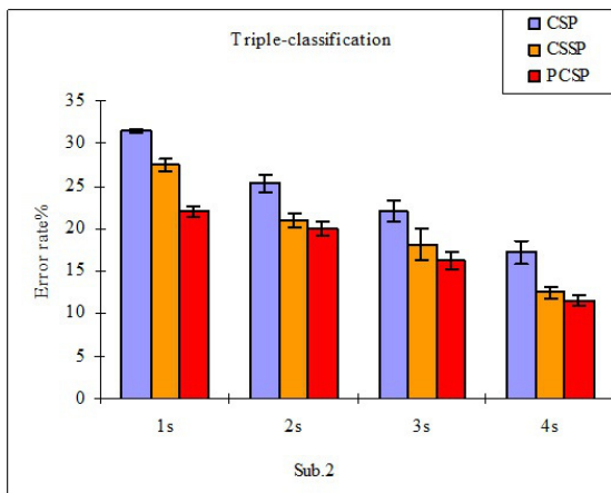
Fig. 10. Error rate and standard deviation of 10-folds cross validation for Sub.2's triple classification
