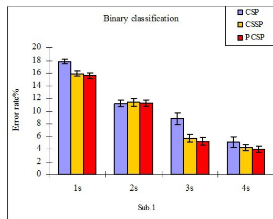
Fig. 7. Error rate and standard deviation of 10-folds cross validation for Sub.1's binary classification
