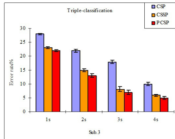
Fig. 12. Error rate and standard deviation of 10-folds cross validation for Sub.3's triple classification
