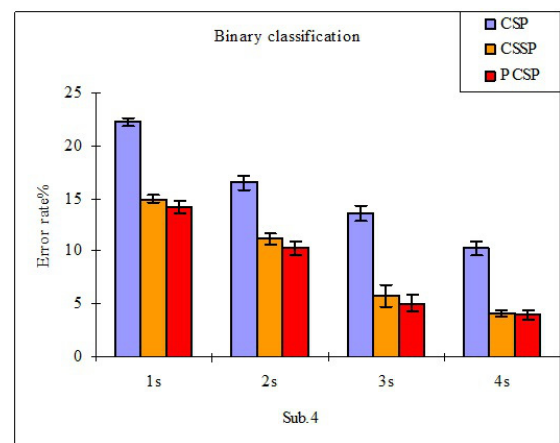
Fig. 13. Error rate and standard deviation of 10-folds cross validation for Sub.4's binary classification
