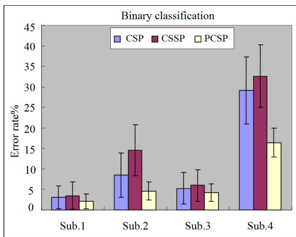
Fig. 6. Error rate and standard deviation of 10-folds cross validation
