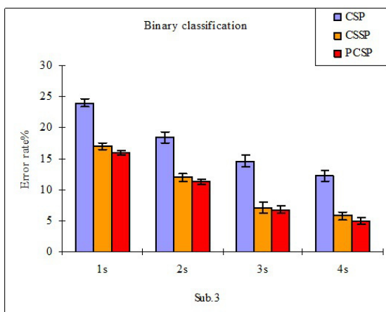
Fig. 11. Error rate and standard deviation of 10-folds cross validation for Sub.3's binary classification
