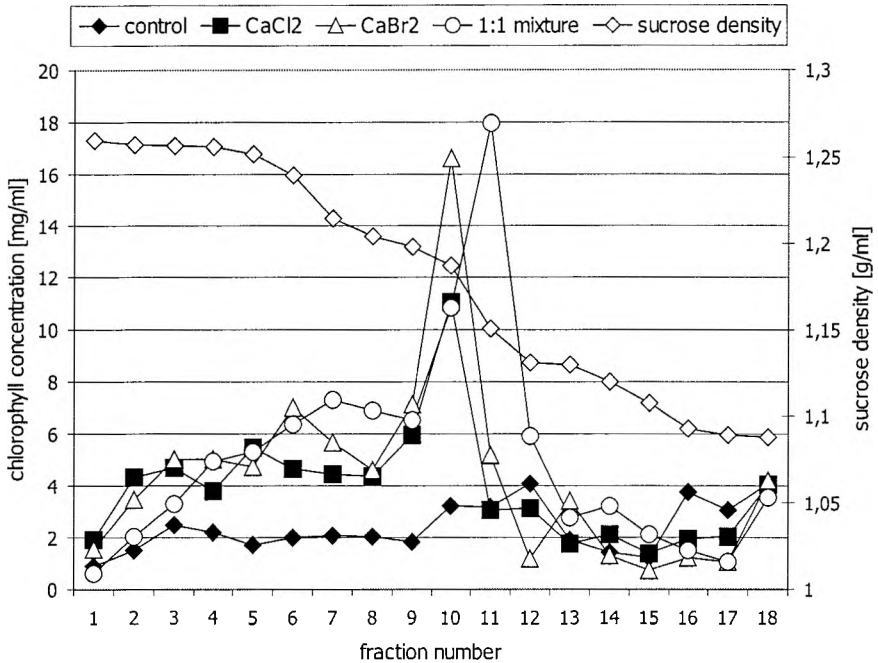
Fig. 2. Sedimentation profiles of chloroplasts (determined as chlorophyll content) from duckweed Lemna minor L. cultivated on control medium as well as on media containing \text{CaCl}_2 , \text{CaBr}_2 and their 1:1 mixture.
