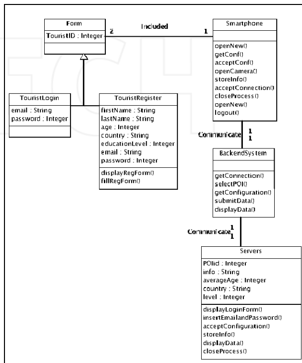
Figure 3. The Class Diagram represents the class structure of AR System
