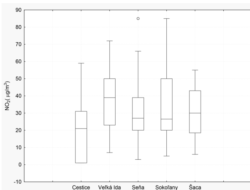
Figure 4. Nitrogen oxides
