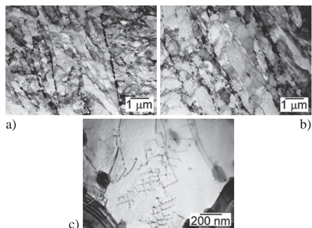
Figure 4 Microstructures observed on the thin films (TEM) in the CGHAZ area of the joint welded using the TBT: a) general morphology of tempered martensite; b) morphology of ferrite subgrains; c) dislocation density in subgrains
