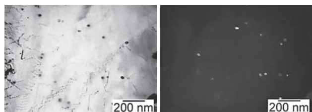
Figure 7 Morphology of NbC carbides observed in the CGHAZ area of the joint welded using the TBT: a) bright visual field; b) dark visual field; c) SAED diffraction pattern of NbC carbides
