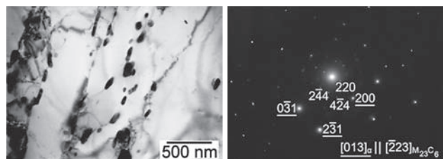
Figure 5 Morphology of M_{23}C_6 carbides observed in the CGHAZ area of the joint subjected to PWHT: a) bright visual field; b) SAED diffraction pattern of M_{23}C_6 carbides: [013]_{\alpha} \parallel [223]_{M_{23}C_6}
