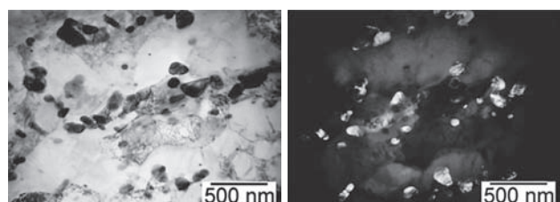
Figure 6 Morphology of M_{23}C_6 carbides observed in the CGHAZ area of the joint welded using the TBT: a) bright visual field; b) dark visual field; c) SAED diffraction pattern of M_{23}C_6 carbides: 112_{\alpha} \parallel [013]_{M_{23}C_6}
