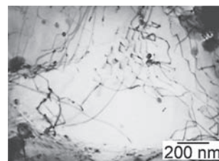
Figure 8 V(CN) (elongated) and NbC (spherical) precipitates in the CGHAZ area of the joint welded using the TBT
