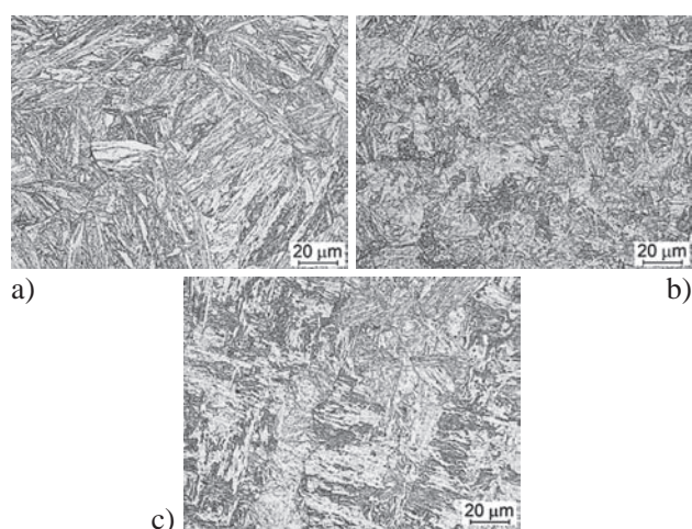
Figure 1 Microstructure of the joint subjected to PWHT: a) PB2 steel parent metal: tempered martensite; b) coarse-grained HAZ (CGHAZ): tempered martensite; c) weld: tempered martensite; etchant: \text{FeCl}_3 , mag. 500x
