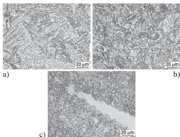
Figure 2 Microstructure of the joint not subjected to PWHT, i.e. welded using the TBT: a) PB2 steel parent metal: tempered martensite; b) CGHAZ: tempered martensite; c) weld: tempered martensite + delta ferrite; etchant: \text{FeCl}_3 , mag. 500x
