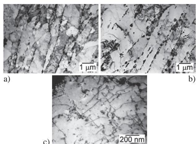
Figure 3 Microstructures observed on the thin films (TEM) in the CGHAZ area of the joint subjected to PWHT: a) general morphology of tempered martensite; b) morphology of ferrite subgrains; c) dislocation density in subgrains
