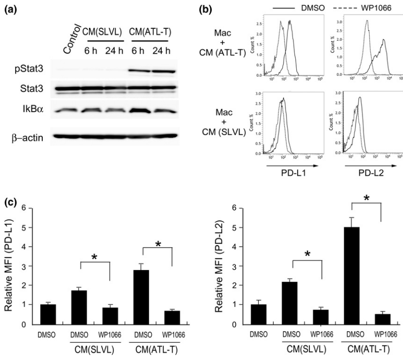
Fig. 3. Stat3 activation and PD-L1/2 upregulation on cultured macrophages. (a) Western blot analysis of pStat3, Stat3 and IκBα expression in cell lysates of cultured macrophages simulated with the conditioned media (CM) of SLVL and ATL-T cells for the indicated times. β-actin was analyzed as a loading control. (b, c) The effect of the Stat3 inhibitor WP1066 on CM-induced overexpression of PD-L1/2 on macrophages (Mac) was tested using flow cytometry (MFI, mean fluorescent intensity; n = 3 for each group). * P -value < 0.05.
