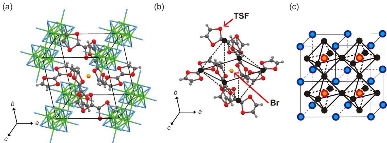
Fig.4. (a) Crystal structure of (\text{TSF}^+)_3[(\text{Mo}_6\text{Br}_{14}^{2-})\text{Br}^-] ( 2 ) depicted in ball and stick style. TSF molecules and bromine anion are depicted as balls (gray, dark gray, red, and orange balls are hydrogen, carbon, selenium, and bromine atoms, respectively.) [\text{Mo}_6\text{Br}_{14}] cluster units are depicted as sticks (green and aqua sticks are molybdenum and bromine atoms, respectively). (b) Unit of octahedral lattice with six TSF molecules and Y = \text{Br} . The center of TSF is represented by a black circle. Y = \text{Br} (orange) is located at the center of the rectangle represented by solid lines. Octahedral lattice of (\text{TSF})_6Y is made by connecting six black circles (solid and dotted black lines). (c) TSF (or TTF) is represented by black balls, Y by orange balls, and Mo clusters by cyan balls to show a schematic view of the antiperovskite structure.
