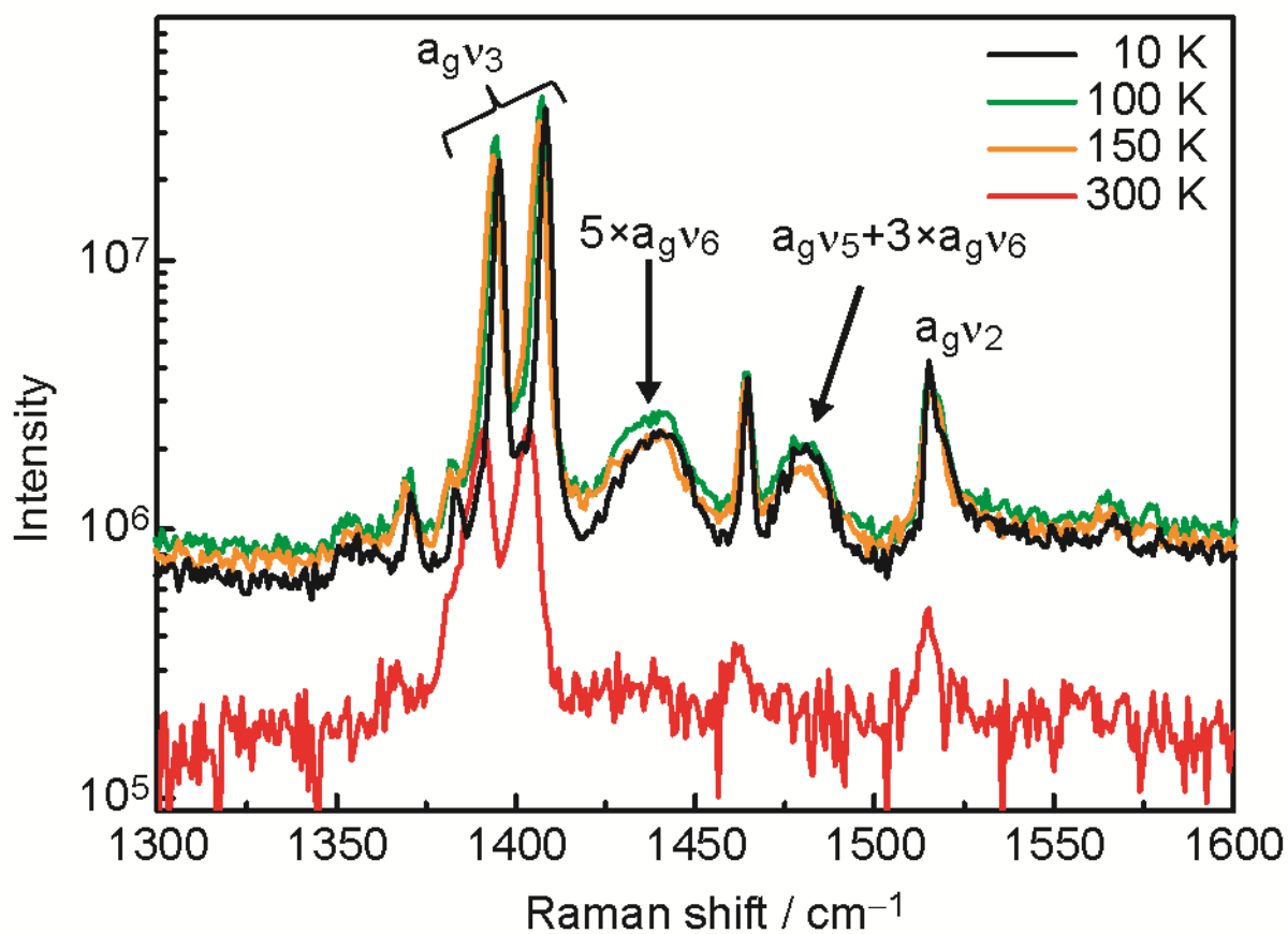
Fig. S5. Temperature dependence of the Raman spectra (300–10 K, 1300–1600 \text{cm}^{-1} ). With the exception of the intensity of overtone and combination bands, the charge sensitive vibration modes ( a_g v_2 , a_g v_3 ) did not show any significant change between 300 and 10 K.
