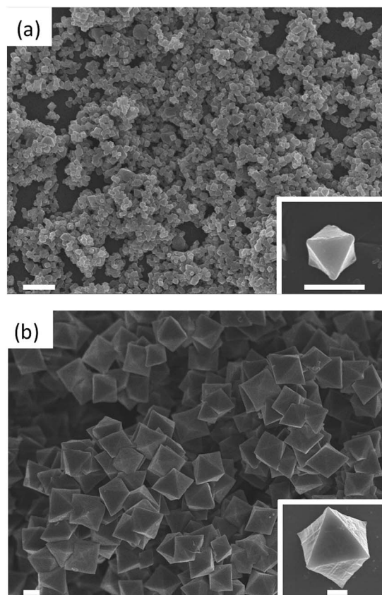
Fig. 2 Representative FESEM of UiO-67-bpy synthesized with 30 eq. (a) and 90 eq. (b) of HAc. Scale bars: 1 μm and 500 nm (inset).
