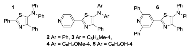
Scheme 1. 5- N -Arylaminothiazoles.
