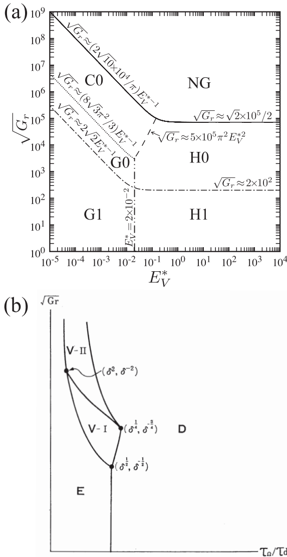
Fig. 5. (a) Same as upper panels of Fig. 1 but for a cross section in E_V^* - \sqrt{Gr} parameter space with the constraints of E_V^{-1} = \tau\Omega and E_V/E_H = 10^{-3} , where E_V^* = 2\pi E_V = 2\pi/(\tau\Omega) . (b) Matsuda's (1980) regime diagram for the similar situation as (a), from his Fig. 10. The symbols D and E denote the direct cell balance and the thermal wind balance of the Earth type, respectively, V-I indicates the region where only the solution in the thermal wind balance of the Venus type (V) exists, V-II indicates that where both the type D solution and the type V solution can exist as multiple equilibrium states, \delta = E_V/E_H , and \tau_0/\tau_d = E_V^* in this panel. Note that the axes in (a) are logarithmic, whereas those in (b) are linear.
