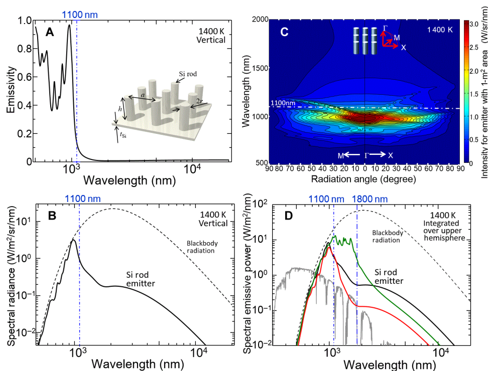
Fig. 1. Theoretical calculation results. (A) Spectral emissivity and (B) spectral radiance of Si rod-array emitter (solid lines) in the direction normal to the surface at 1400 K with a = 500 nm, h = 450 nm, r = 110 nm, and t_{\text{Si}} = 50 nm. The inset in (A) illustrates the emitter structure and parameters. (C) Radiation angle dependence of emission intensity at 1400 K for the emitter with a 1\text{-m}^2 area. (D) Radiation spectra of Si rod-array emitters at 1400 K integrated over the upper hemisphere with structural parameters a = 500 nm, h = 450 nm, r = 110 nm, and t_{\text{Si}} = 50 nm (solid black line); a = 600 nm, h = 600 nm, r = 105 nm, and t_{\text{Si}} = 0 nm (solid red line); and a = 700 nm, h = 800 nm, r = 190 nm, and t_{\text{Si}} = 0 nm (solid green line). The blackbody spectrum at 1400 K integrated over the upper hemisphere (dashed line) and the irradiance of sunlight at AM1.5G (gray line) are also plotted.
