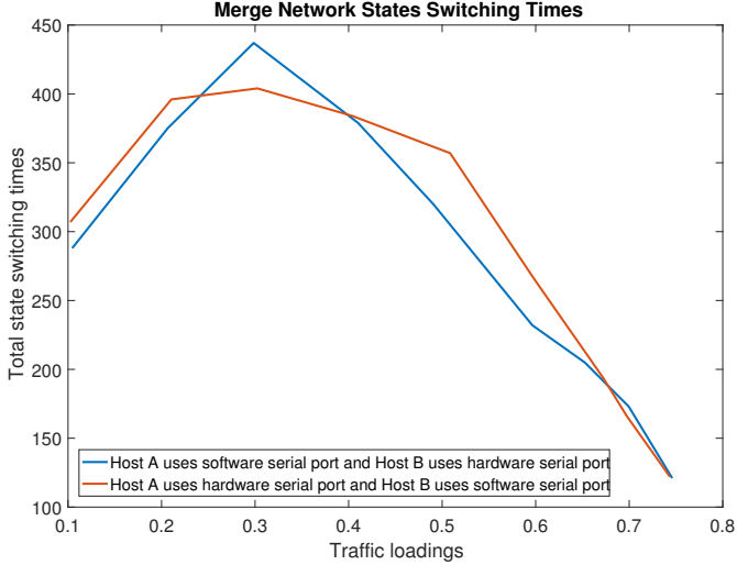
Figure 8.14. Total state switching times.
