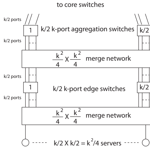
Figure 6.3. Merge network applied to pod in a fat-tree .
