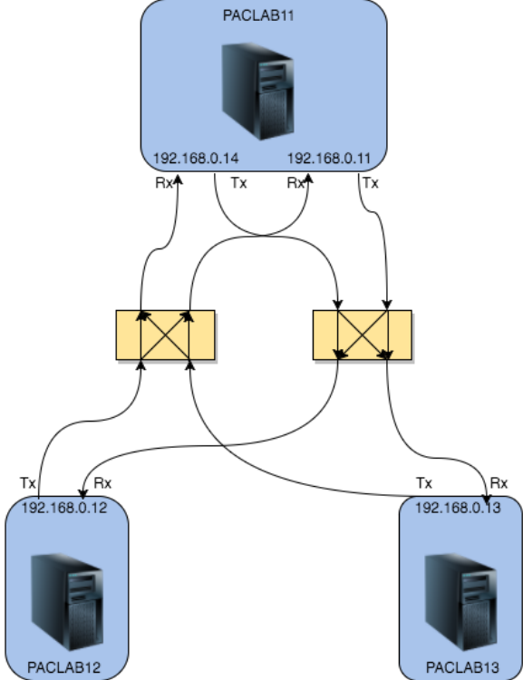
Figure 8.1. A 2 × 2 merge network implemented with two 2 × 2 optical switches.
