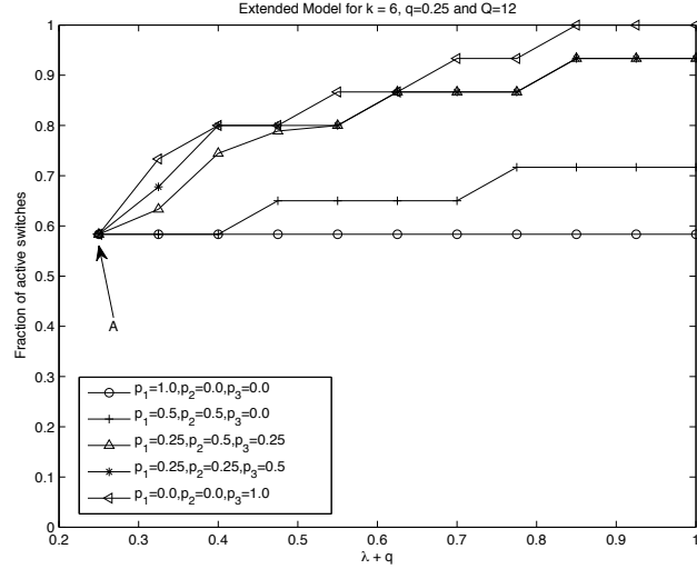
Figure 3.3. Extended model with high external connectivity.
