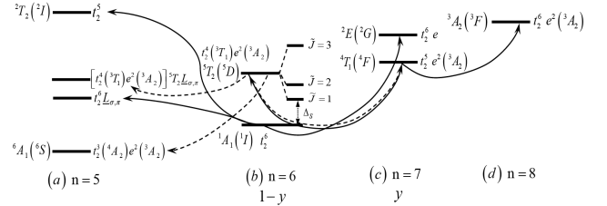
Fig. 3: Multielectron terms of CoO_6 -cluster with five (a), six (b), seven (c) and eight (d) electrons above the configuration d^0(Co)p^6(O) . For stoichiometric GdCoO_3 at T = 0 , only the lowest LS d^6 {}^1A_1 term is occupied, all other terms unoccupied, but for nonstoichiometric crystal Gd^{3+}Co_{1-y}^{3+}Co_y^{2+}O_{3-\delta}^{2-} ( y = 2\delta ) also HS d^7 {}^4T_1 is occupied with filling factors f_{Co^{3+}}^{LS} = 1 - y and f_{Co^{2+}}^{HS} = y respectively. A set of Co^{3+} HS states split by spin-orbital interaction is above the LS term with the spin gap \Delta_S = E_{HS} - E_{LS} . Electron addition d^6 \rightarrow d^7 and d^7 \rightarrow d^8 excitations forming the bottom of the conduction band and electron removal d^6 \rightarrow d^5 , d^7 \rightarrow d^6 excitations forming the top of valence band are shown by solid lines. The dashed lines indicate the excitations responsible for the formation of band states upon the Co^{3+} HS thermal population.
