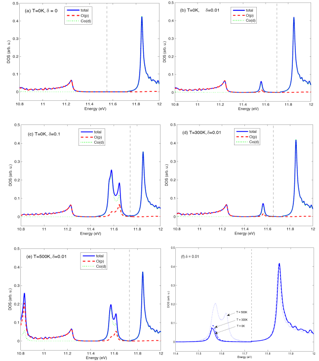
Fig. 4: (Color online) Total and partial DOSs for the stoichiometric GdCoO_3 at T = 0 K (a) and for the nonstoichiometric GdCoO_{3-\delta} compound at T = 0 (b, c), T = 300 (d) and 500 K (e), calculated within the LDA+GTB. At T = 0 GdCoO_3 is the insulator with the gap E_g \approx 0.5 eV. At \delta \neq 0 the in-gap band appears below the conductivity band with the temperature dependent spectral weight and bandwidth. The dashed line shows the chemical potential. On the last figure (f) we summarized and imposed the total DOSs in the vicinity of chemical potential for three different temperatures T = 0, 300 and 500 K (solid, dashed and dotted line respectively) and fixed \delta = 0.1 on an enlarged scale.
