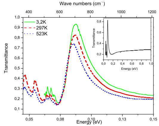
Fig. 1: (Color online) The transmittance spectrum of GdCoO_{3-\delta} , measured at T = 3.2 K (solid line), T = 297 K (dashed line) and T = 523 K (dark circles). The room temperature transmittance in the wide energy region is shown in the insert to demonstrate the absence any features at high energy.
