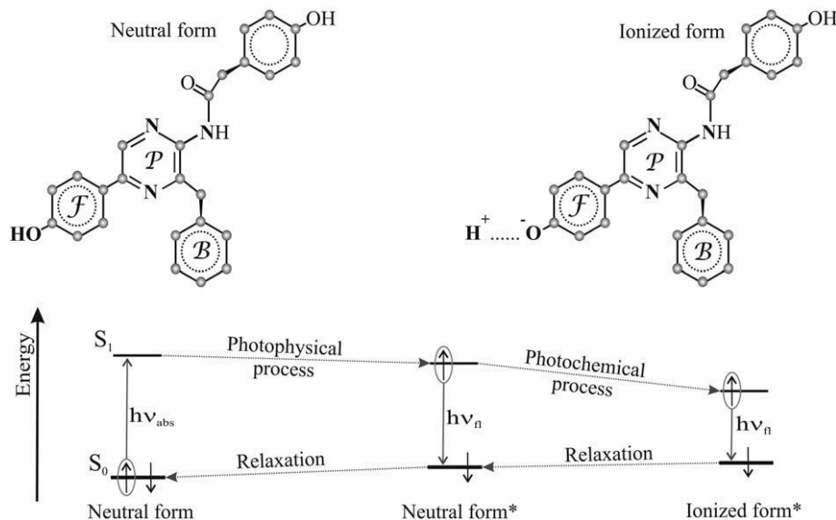
Fig. 1. Scheme of photophysical and photochemical processes in coelenteramide and coelenteramide-containing fluorescent proteins.
