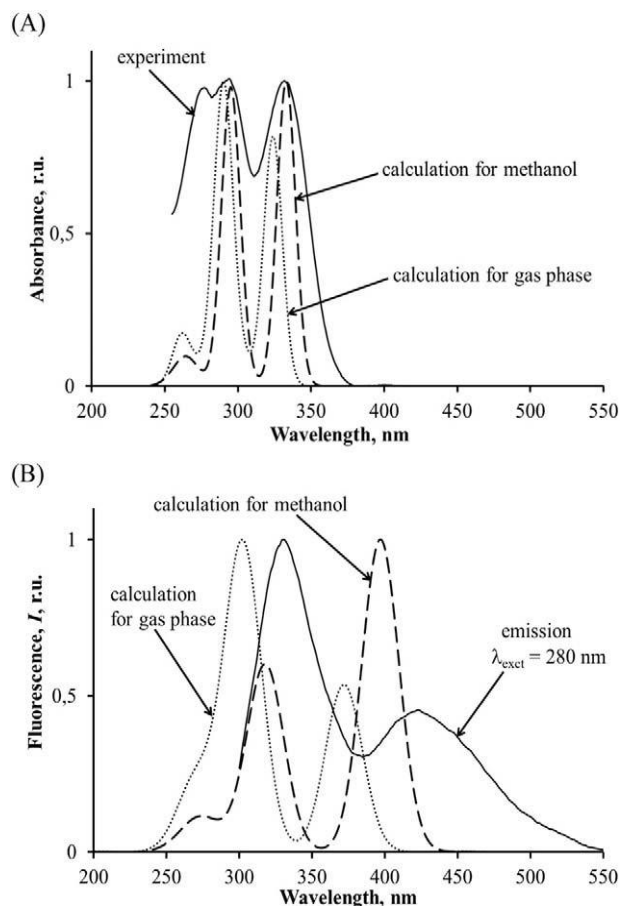
Fig. 5. Experimental and theoretical absorption (A) and fluorescence (B) spectra of coelenteramide, C_{CLM}=2,2-10-\epsilon -M, methanol. Calculations were provided for gas phase and methanol by SMD*/TD//B3LYP/cc-pVDZ. Theoretical spectra were simulated by Gaussian convolution with full width at half maximum: absorption spectra of 15 nm, fluorescence spectra of 30 nm.
