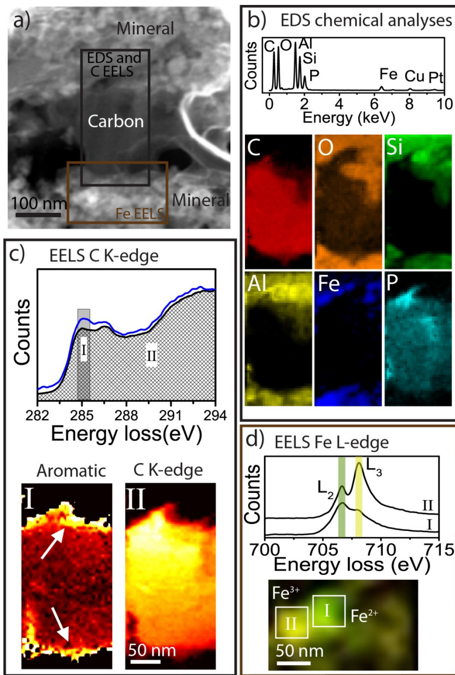
Figure 4. STEM nanoscale analyses of a biochar organo-mineral interface of GWS a) STEM-HAADF image of the organo-mineral interface. The two rectangular regions of interest are where chemical analyses were performed. b) Top: EDS spectrum image data obtained from the upper region of interest in a). Bottom: EDS maps show the elemental distribution of the C, O, Si, Al, Fe, and P. Cu and Pt signals in the EDS spectrum come from the TEM grid and the Pt protection layer, respectively. c) EELS C K-edge spectra (top) and maps (bottom) obtained from the upper region of interest in a). The upper (blue) spectrum has been slightly shifted upwards after normalisation to highlight the differences at c.a. 285 eV. Map I was obtained using the energy window I at 285 eV and
