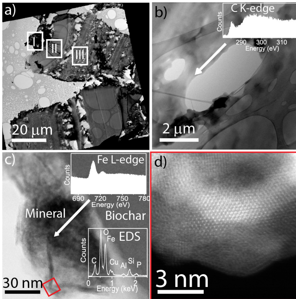
Figure 2. TEM analyses of the organo-mineral interface in RCBS. a) Low magnification BF-TEM image showing a general view of the microtomed sample. b) BF-TEM image showing details of large macropores present between the organo-mineral layer and the biochar (regions III and II in a). Inset is a C K-edge EEL spectrum from the carbon-rich matrix. c) BF-STEM image of the complex micro-agglomerate layer that has formed on the surface of the biochar. Insets: top Fe L 2,3 -edge EEL spectrum from the region arrowed – edge shape is typical of Fe 3 O 4 ; bottom EDS spectrum from the same region as EELS showing strong Fe and O signals; Al, Si, and P were also detected. d) Atomic resolution STEM-HAADF detail of the boxed region (red) in c) showing interplanar spacings consistent with Fe 3 O 4 .
