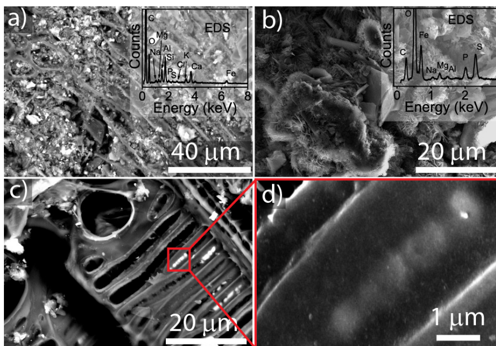
Figure 5. a) and b) Secondary electron SEM micrographs of the surface of the composted WC biochar partially coated with both organic and inorganic matter. The insets show EDS spectra collected over the field of view. c) and d) are SE images of the surface of the WC in a region with high concentration of calcium (bright areas).
