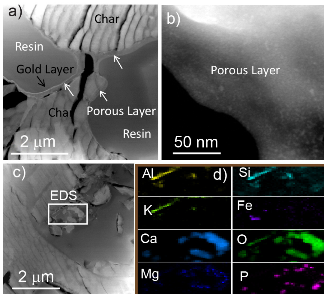
Figure 6. STEM-HAADF images (60 kV) of a microtomed slice from a composted Kon-Tiki biochar (WC). a) Biochar particle embedded in resin showing the porous layer on top of the biochar. The large resin filled pore on the right shows poor coverage with sputtered gold, due to a shadowing effect. The more exposed pore (top left) shows better coverage. b) Detailed view of the porous layer. c) Another sectioned region showing a group of mineral particles at the surface of WC. d) X-ray maps (EDS) of the boxed region in c).
