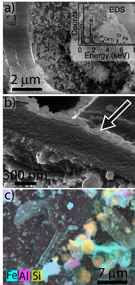
Figure 1. SEM secondary electrons imaging of the carbon matrix-organo-mineral interface of RCBS. a) Inorganic precipitates inside a large elliptical pore of woody biochar; inset shows EDS spectrum collected from the whole area inside the pore. b) Detail of the organo-mineral layer (bright layer indicated by the arrow) formed on the pore walls; c) Image of a pore covered with micron and sub-micron sized mineral and organo-mineral particles and EDS elemental map, showing Fe, Al and Si distributions.
