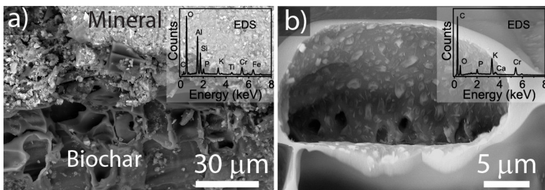
Figure 3. SEM SE images of the organo-mineral/carbon matrix interface in GWS. a) SE image of the organo-mineral layer on the particle surface (top) and the underlying biochar porous matrix (bottom). The inset shows the EDS analysis of the organo-mineral layer. b) An image of an internal pore coated in organic and mineral matter – EDS spectrum of this area is shown inset.
