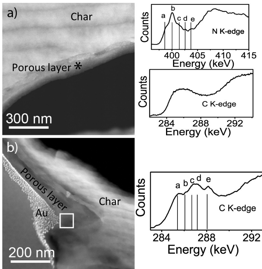
Figure 7. STEM - HAADF images (60 kV) and N K and C K-EEL spectra collected using cold stage microscopy of composted WC biochar. a) Left – STEM-HAADF image showing a cross section through the porous layer. N K-edge spectra were acquired (right) at the point marked with *. Peaks due to N-containing functional groups are observed and marked a-e (see text for detailed explanation). Centre right –C K-EEL spectrum taken from the biochar matrix and shows a broad peak from 285.1 eV to 287.3 eV indicating a low concentration of C/O functional groups and a high concentration of amorphous carbon. b) Left - STEM-HAADF image of another region of the porous layer. Bottom right - C K-edge spectra obtained from the boxed region in b). Peaks due to carbon-containing functional groups in the EELS are labelled a to e: a-285.1 eV → aromatic, b-286.1 eV → aromatic with side chain, c-286.8 eV → ketone, d-287.3 eV → aliphatic, and e-288.1eV → carboxyl/amine carbon.
