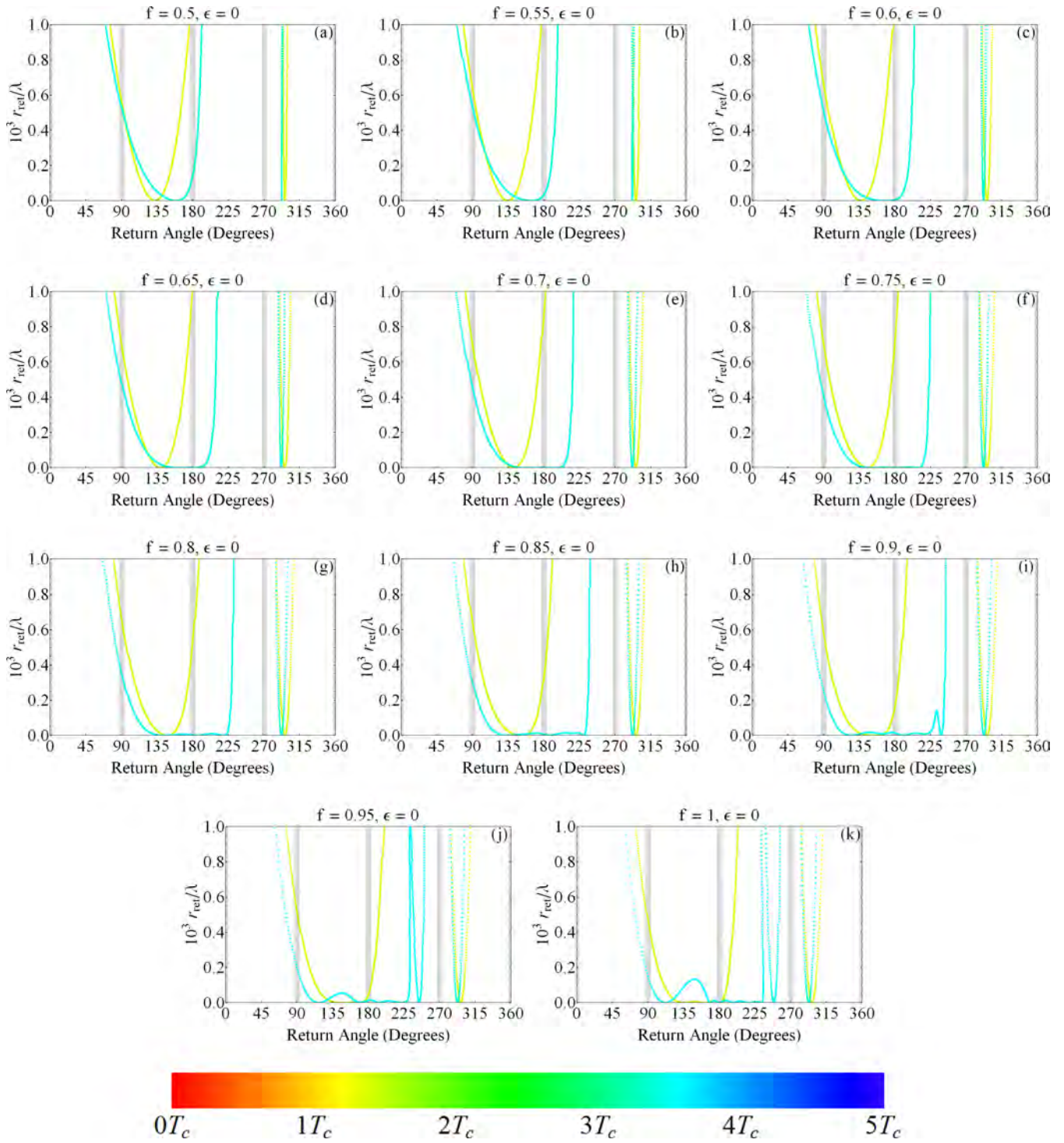
FIG. 19. Return distance ( r_{\text{ret}} ) to the nucleus as a function of azimuthal return angle for the second and fifth harmonics in the scaled-field region of f = 0.5 to 1 in steps of f = 0.05 .
