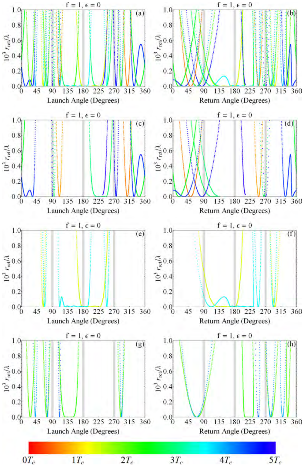
FIG. 8. Return distance ( r_{\text{ret}} ) to the nucleus as a function of azimuthal launch (left column) and return (right column) angle for entire set of harmonics and comparable harmonics at f = 1 and \epsilon = 0 .
