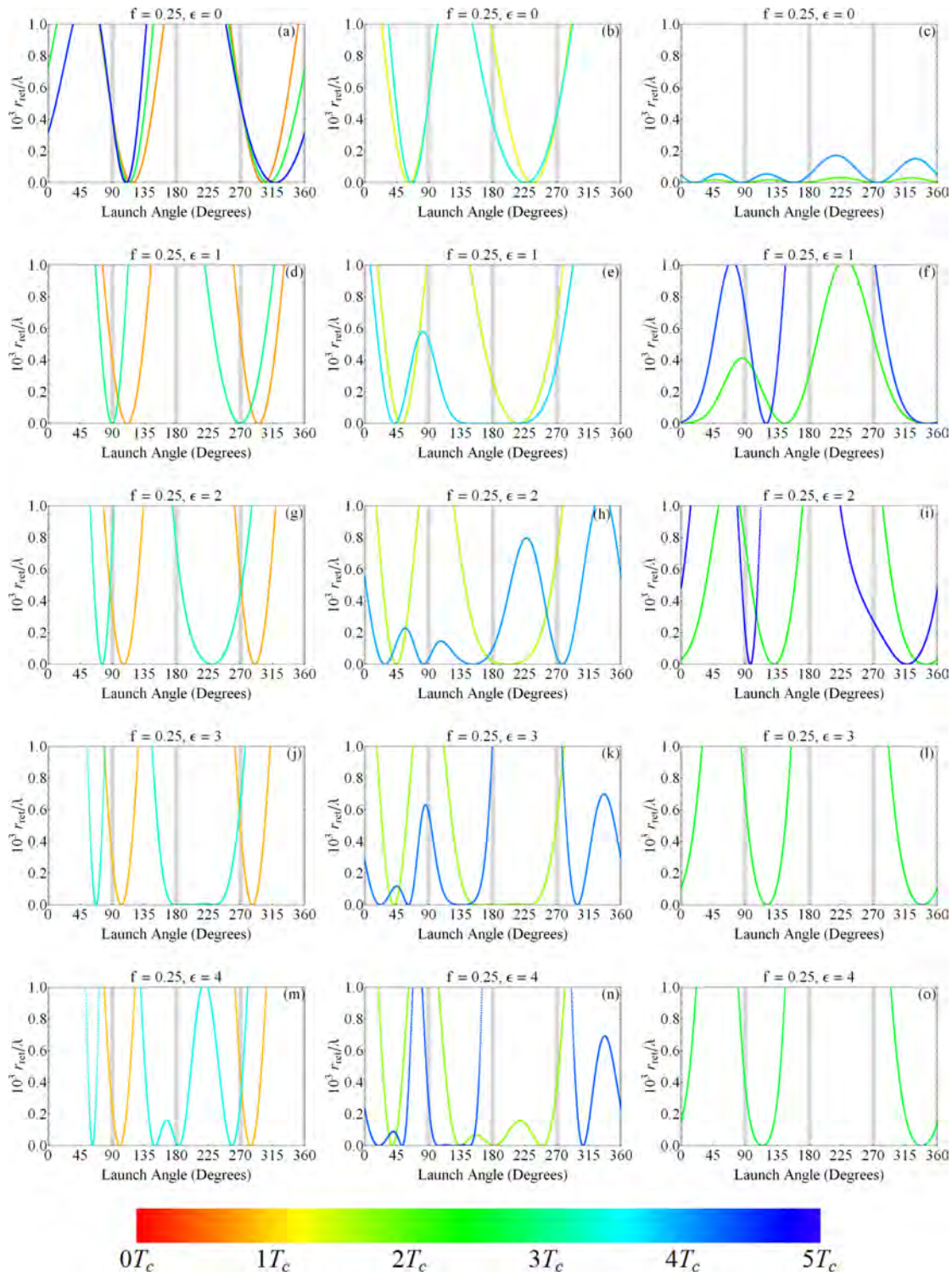
FIG. 12. Return distance ( r_{ret} ) to the nucleus as a function of azimuthal launch angle at f = 0.25 as the scaled energy is increased in integer increments from \epsilon = 0 to 4. In the figure, scaled energy increases from top to bottom. The left column shows the first, fourth, and seventh harmonics, the middle column shows the second and fifth harmonics, and the right column shows the third and sixth harmonics.
