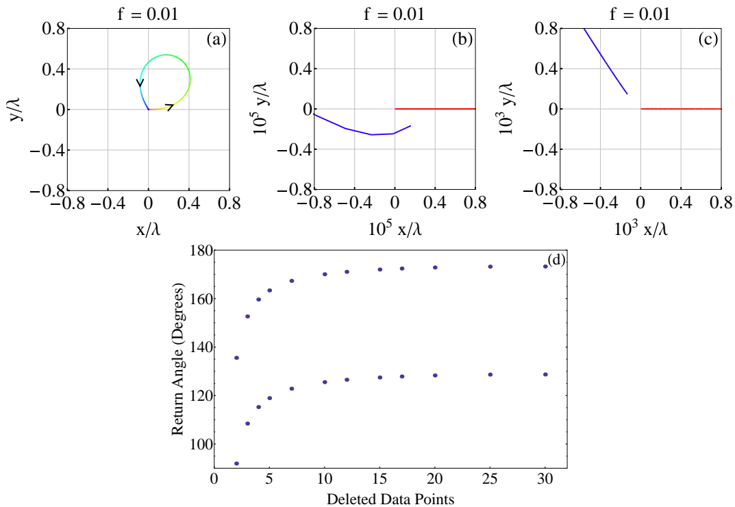
FIG. 2. Panels (a), (b), and (c) show an example of a seemingly closed orbit for f = 0.01 , \epsilon = 0 , and \phi = 0^\circ . The color of the orbit evolves with time from launch (red) to return (blue) as denoted by the direction of the arrows which show the launch and return branches of the orbit path. Panel (a) is the entire orbit, panel (b) zooms in on the region around the nucleus to reveal the problem with using the closest point for calculating the return angle. Panel (c) shows the orbit minus the last nineteen points to reveal a good estimate of the return angle. Note panel (b) is magnified two orders of magnitude further than panel (c). Panel (d) shows the calculated return angle as a function of the number of data points omitted from the closest pass to the nucleus. Two orbits of high curvature near the nucleus from Fig. 9 were considered. After \sim 20 points from the nucleus, the return angle stabilizes and was therefore utilized as our condition for the calculation of the return angle.
