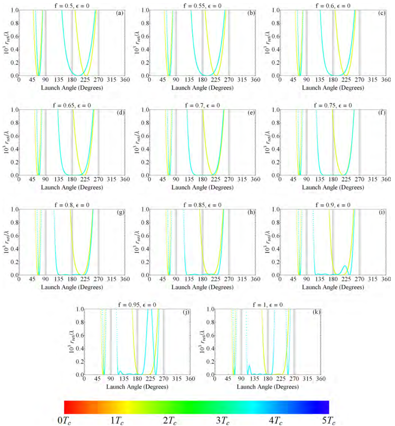
FIG. 18. Return distance ( r_{ret} ) to the nucleus as a function of azimuthal launch angle for the second and fifth harmonics in the scaled-field region of f = 0.5 to 1 in steps of f = 0.05 .
