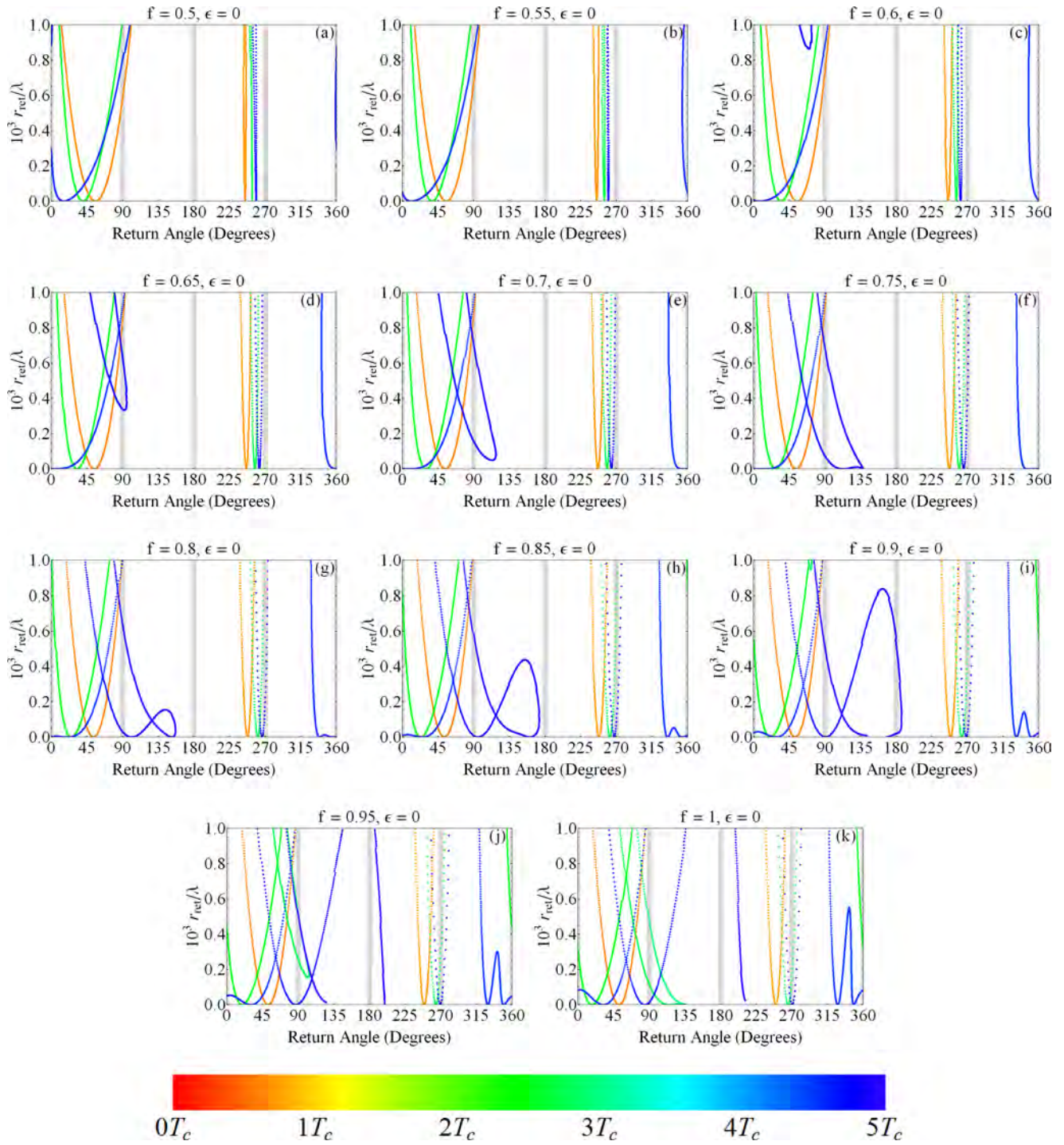
FIG. 17. Return distance ( r_{rel} ) to the nucleus as a function of azimuthal return angle for the first, fourth, and seventh harmonics in the scaled-field region of f = 0.5 to 1 in steps of f = 0.05 .
