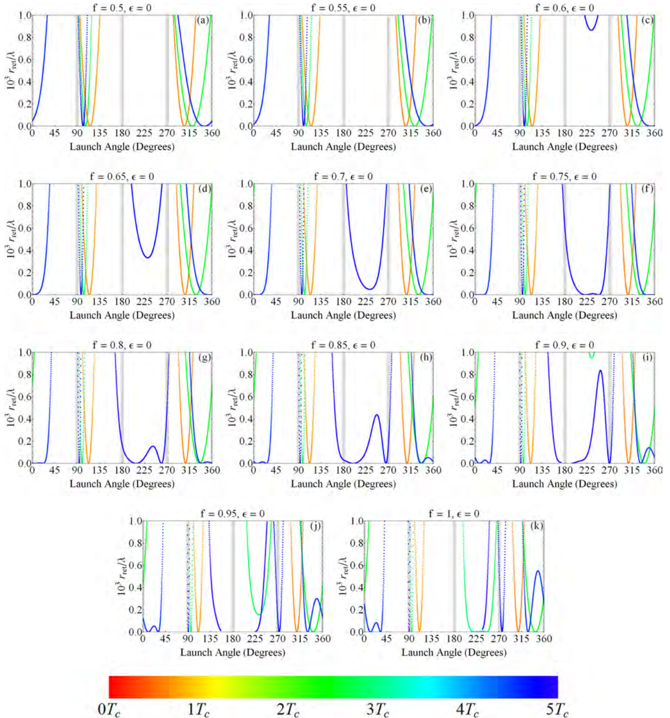
FIG. 16. Return distance ( r_{\text{rel}} ) to the nucleus as a function of azimuthal launch angle for the first, fourth, and seventh harmonics in the scaled-field region of f = 0.5 to 1 in steps of f = 0.05 .
