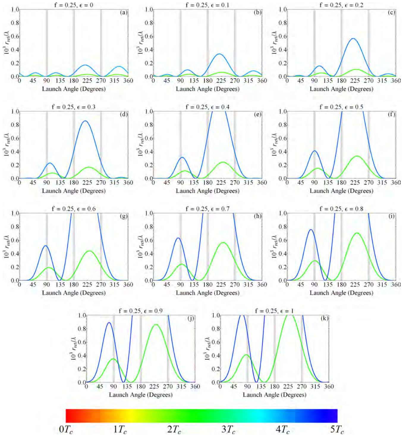
FIG. 22. Return distance ( r_{\text{ret}} ) to the nucleus as a function of azimuthal launch angle for the third and sixth harmonics at f = 0.25 for varying scaled energy between \epsilon = 0 and 1 in 0.1 steps.
