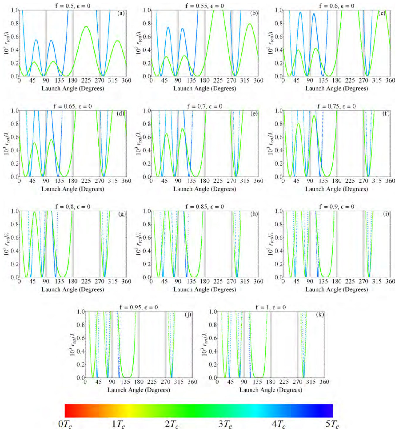
FIG. 20. Return distance ( r_{\text{ret}} ) to the nucleus as a function of azimuthal launch angle for the third and sixth harmonics in the scaled-field region of f = 0.5 to 1 in steps of f = 0.05 .
