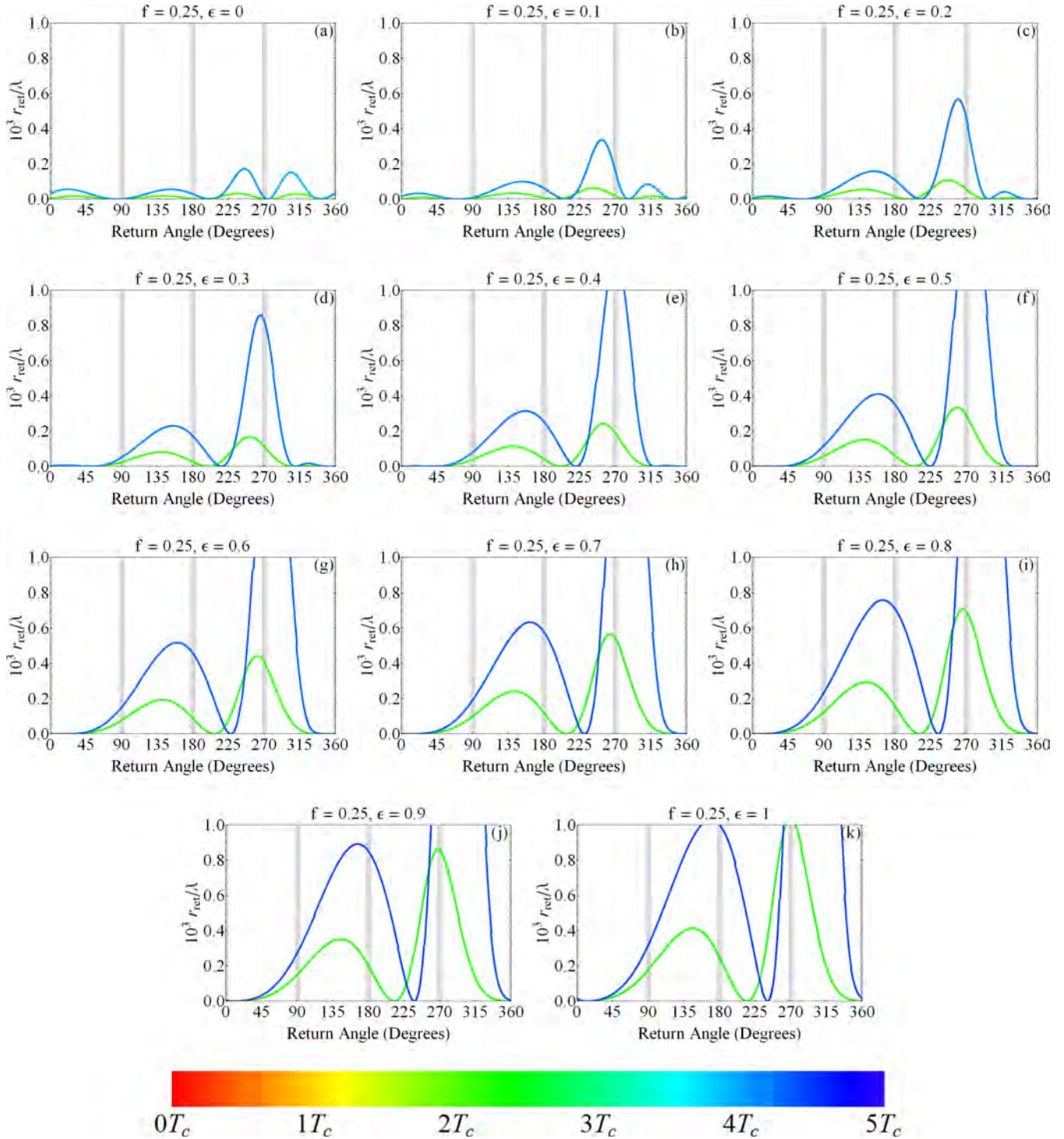
FIG. 23. Return distance ( r_{\text{ret}} ) to the nucleus as a function of azimuthal return angle for the third and sixth harmonics at f = 0.25 for varying scaled energy between \epsilon = 0 and 1 in 0.1 steps.
