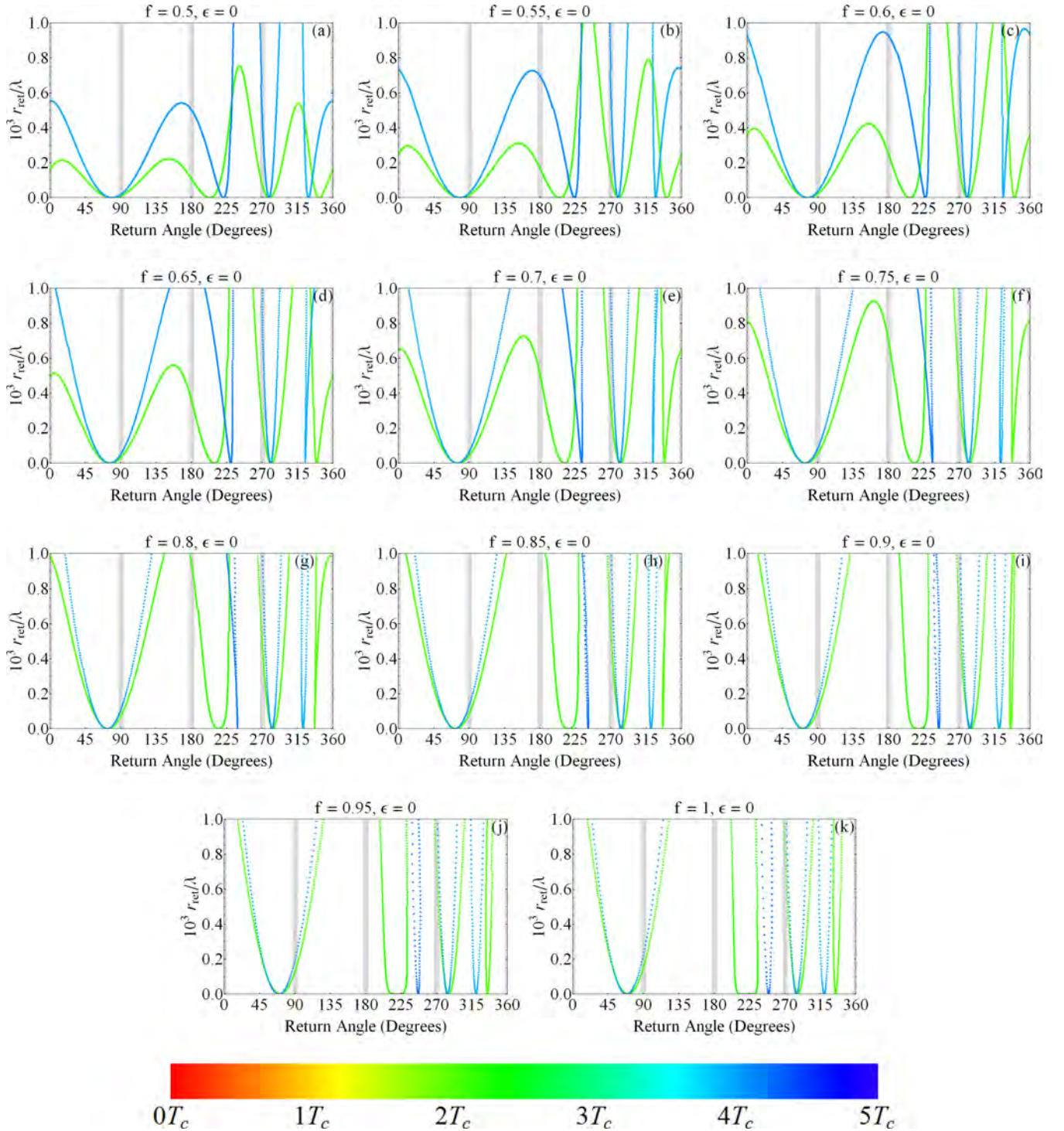
FIG. 21. Return distance ( r_{\text{ret}} ) to the nucleus as a function of azimuthal return angle for the third and sixth harmonics in the scaled-field region of f = 0.5 to 1 in steps of f = 0.05 .
