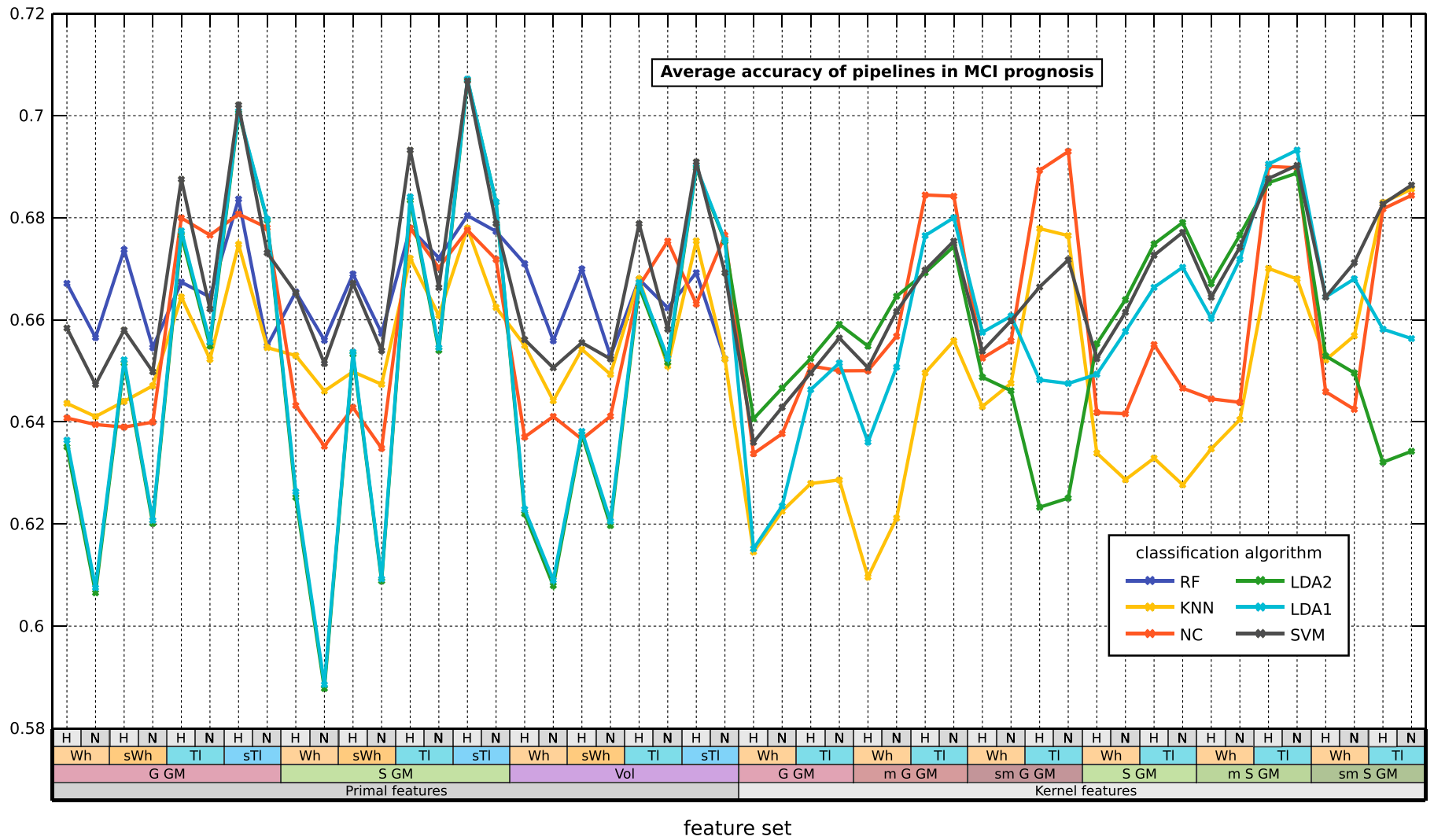
Fig. B.14. Average accuracies of MCI prognosis pipelines measured using 4x6cv with 160 subjects. See key in Fig. B.12.
