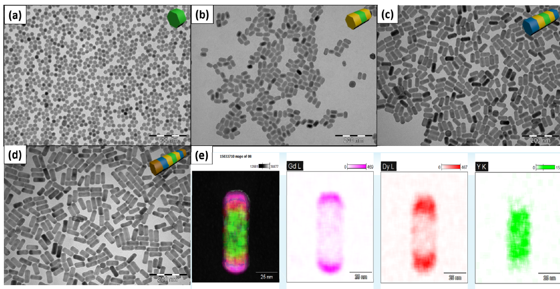
Figure 2. TEM images of the UCNPs nanospheres (a) and nanorods (b-d) with different aspect ratio and different materials through longitudinal epitaxial growth. (a) UCNPs core nanospheres \text{NaYF}_4:\text{Yb,Er} ; (b) three-section \text{NaYF}_4:\text{Yb,Er-NaYF}_4 nanorods by growth of \text{NaYF}_4 ; (c) five-section \text{NaYF}_4:\text{Yb,Er-NaYF}_4\text{-NaDyF}_4 nanorods by growth of \text{NaDyF}_4 ; (d) seven-section \text{NaYF}_4:\text{Yb,Er-NaYF}_4\text{-NaDyF}_4\text{-NaGdF}_4 nanorods by growth of \text{NaGdF}_4 ; (e) HAADF-STEM image with elemental mapping of the seven-section \text{NaYF}_4:\text{Yb,Er-NaYF}_4\text{-NaDyF}_4\text{-NaGdF}_4 nanorod.
