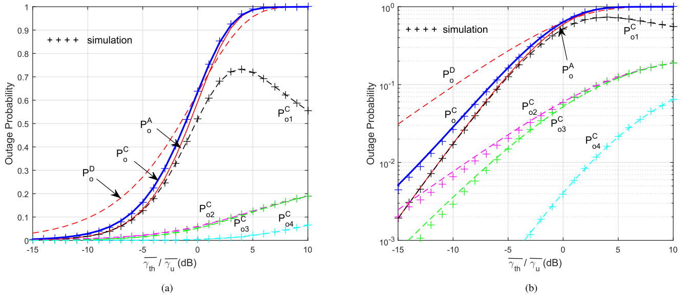
FIGURE 9. Component outage probabilities and overall outage probability of the cooperative system vs. outage of direct transmission and of the Alamouti transmission, assuming \bar{\gamma}_{ij} = \bar{\gamma}_u . Solid curves and dashed curves show the numerical analysis, while plus sign markers indicate the simulation results. (a) Linear scale. (b) Logarithmic scale.
