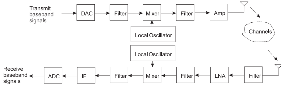
FIGURE 3. Component power model for energy efficiency analysis.
