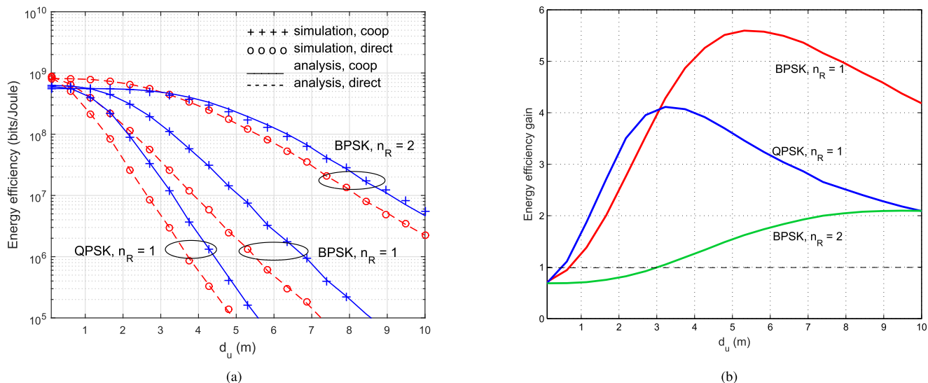
FIGURE 11. Numerical and simulated EE and G_{EE} of the cooperative communication versus those in the direct transmission. (a) EE . (b) G_{EE} .
