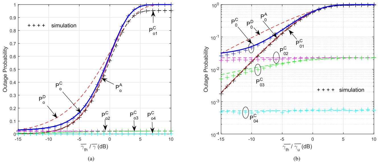
FIGURE 10. Component outage probabilities and overall outage probability of the cooperative system vs. outage of direct transmission and of the Alamouti transmission, assuming \bar{\gamma}_{ij} = 10 dB. Solid curves and dashed curves show the numerical analysis, while plus sign markers indicate the simulation results. (a) Linear scale. (b) Logarithmic scale.
