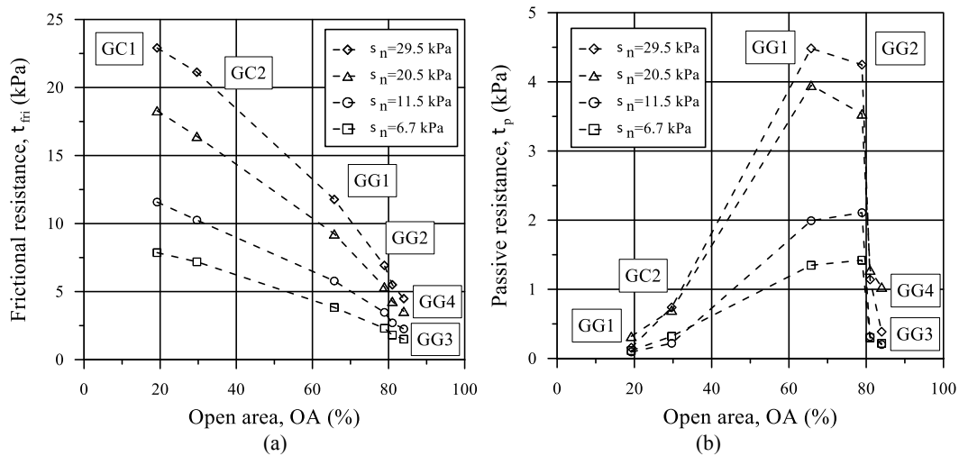
Figure 6: Computation of (a) frictional resistance ( \tau_{fr} ) and (b) passive resistance ( \tau_p ) at different opening area (OA) of different geosynthetics (data sourced from Biabani & Indraratna, 2015).
