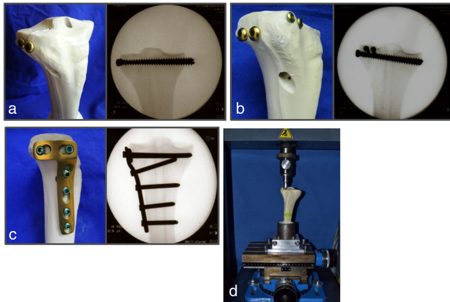
Fig. 2 Types of osteosyntheses. The fractures were stabilized with three different osteosyntheses: a 2 screws, b 4 screws in the jail technique, and (c) lateral angle stable L-buttruss plate. After stabilization an axial load was applied by an indenter on the lateral tibial plateau (d)
