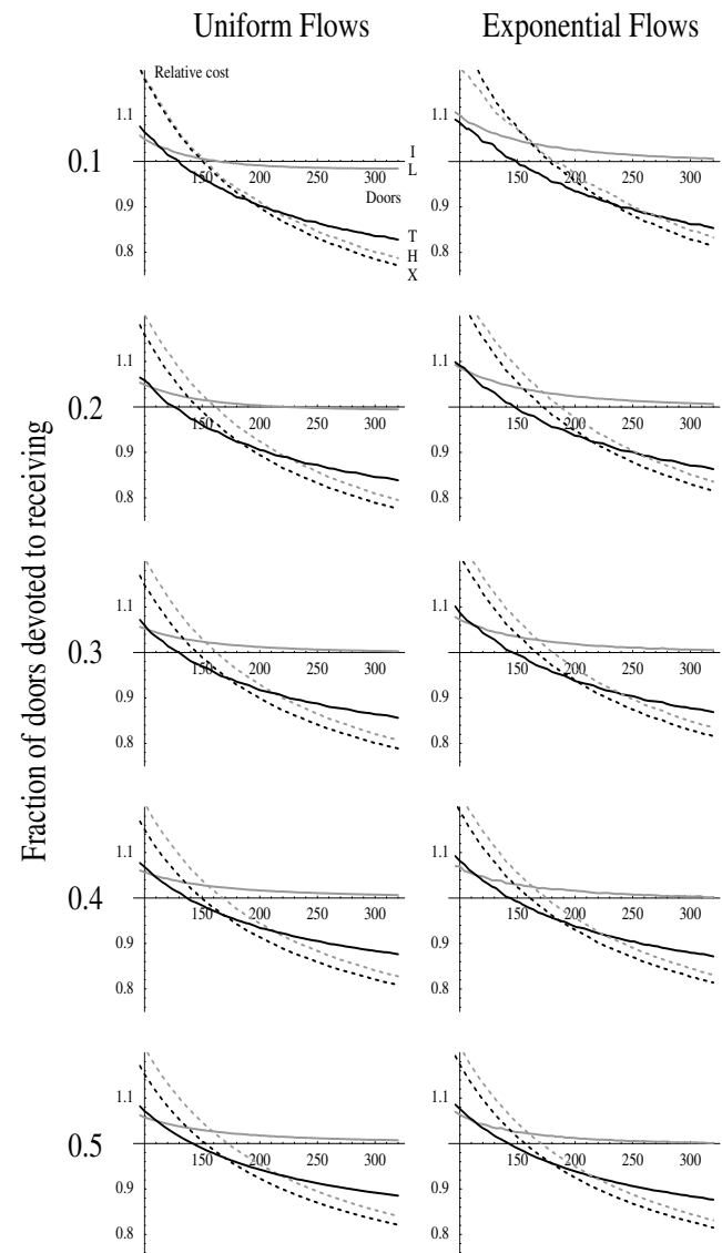
Figure 8 Results of the Experiment Note. Curves represent the cost of each shape relative to the I. Thus, the x-axis represents the cost of the I; the solid black curve represents the cost of the T; the dashed black curve represents the X; the solid gray curve represents the L; and the dashed gray curve represents the H, as indicated in the upper left-hand plot.
