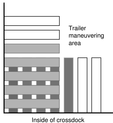
Figure 1 An Inside Corner that Constricts Parking Space for Trailers Note. This makes some door positions unusable (marked in light and dark gray). As a result, a dock with an inside corner must be larger to provide the desired number of usable doors.
