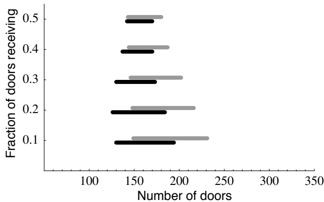
Figure 7 Regions for Which the T-Shape Is Best Note. The black bars indicate regions for which the T-shape is most labor-efficient when freight flows are uniform, and gray bars show the same for exponential freight flows. To the left of the bars the I-shape is best, and to the right the X is best.
