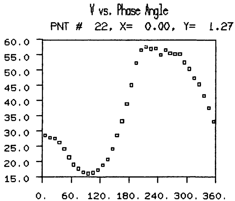
Fig. 14. Ensemble Averaged Velocities in the Flow Over an Oscillating Airfoil: LDV Data. M = 0.3 , k = 0.05 , x/c = 0.0 , y/c = 0.167 , z/c = 0.0 , \alpha = 10^\circ - 10^\circ \sin \omega t
