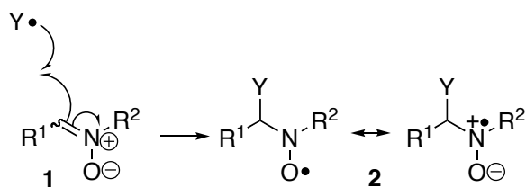
Scheme 1 Spin trapping with nitrones
