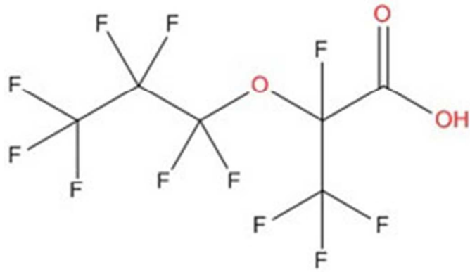
Figure 1. Chemical structure of 2,3,3,3-tetrafluoro-2-(heptafluoropropoxy)-propanoate.
