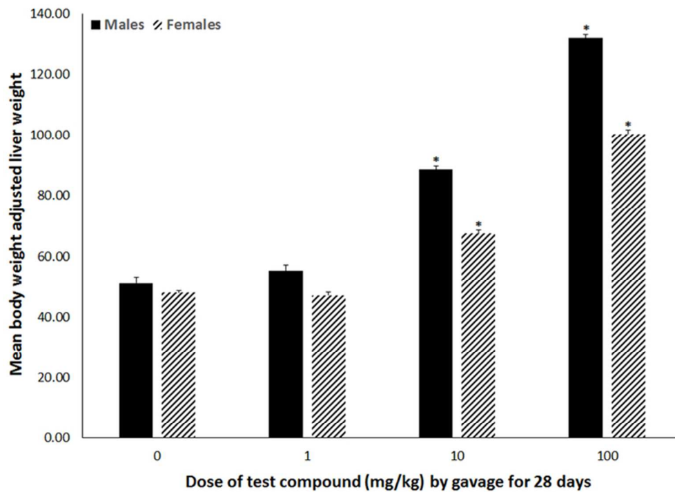
Figure 3. Relative liver weights (absolute liver weight adjusted for body weight; mean \pm SD) of male or female C57Bl/6 mice given 2,3,3,3-tetrafluoro-2-(heptafluoropropoxy)-propanoate via gavage for 28 days. Livers were collected one day after exposure ended. *indicates a statistically significant increase in relative liver weight relative to the 0 mg/kg group of the matching sex ( p < 0.05 ).
