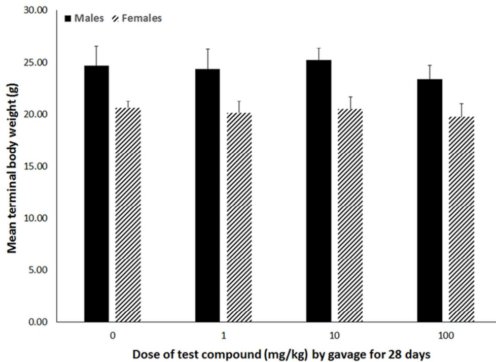
Figure 2. Body weights (mean \pm SD) of male or female C57Bl/6 mice given 2,3,3,3-tetrafluoro-2-(heptafluoropropoxy)-propanoate via gavage for 28 days. No statistically significant differences in mean body weights collected at study terminus (one day after exposure ended) were associated with test compound exposure.
