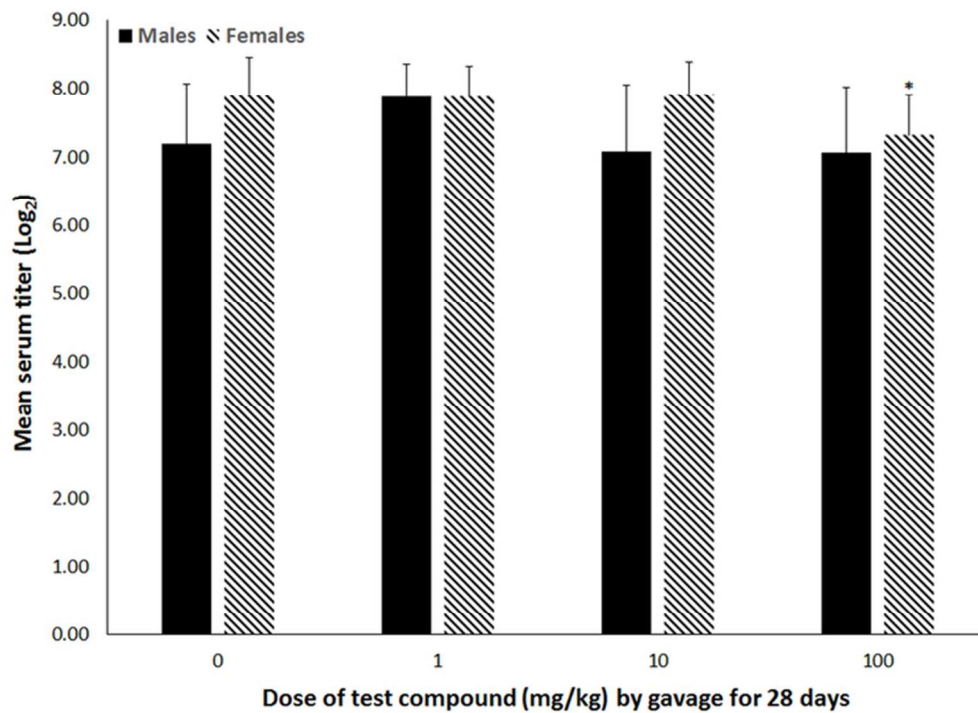
Figure 5. Antigen-specific IgM antibody production (mean \pm SD) of male or female C57Bl/6 mice given 2,3,3,3-tetrafluoro-2-(heptafluoropropoxy)-propanoate via gavage for 28 days. IgM serum titers were measured in archived sera that had been collected from animals one day after exposure ended. *indicates a statistically significant reduction in IgM serum titer relative to the 0 mg/kg group of the matching sex ( p < 0.05 ).
