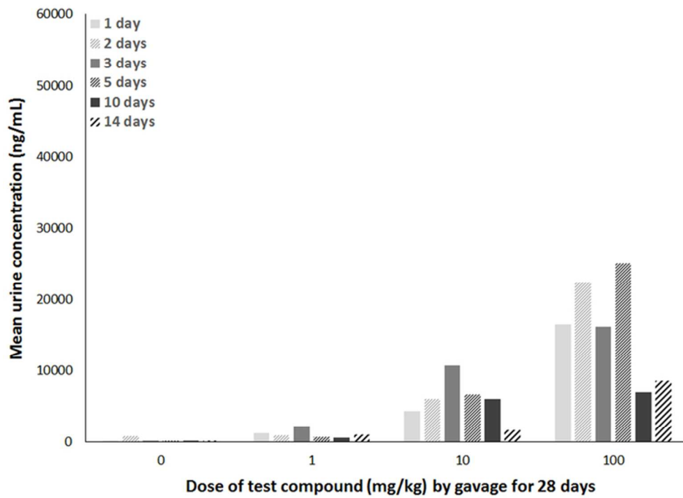
Figure 7. Urine concentrations (mean) of male or female C57Bl/6 mice given 2,3,3,3-tetrafluoro-2-(heptafluoropropoxy)-propanoate via gavage for 28 days. Urine samples were collected after 1, 2, 3, 5, 10, and 14 days of exposure. A) Males. B) Females. Samples are pooled samples of three animals/sex/cage and two pooled samples/dose; sample sizes are therefore N = 1 or 2/dose depending on the quantity of urine non-invasively excreted on a particular sample collection day.
