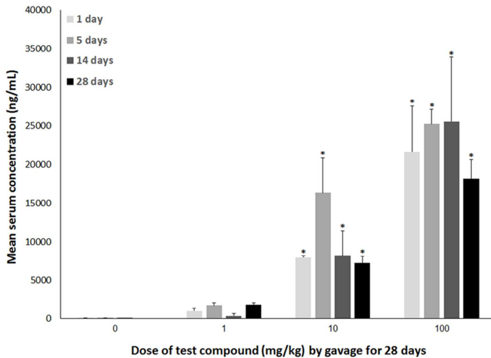
Figure 6. Serum concentrations (mean \pm SD) of male or female C57Bl/6 mice given 2,3,3,3-tetrafluoro-2-(heptafluoropropoxy)-propanoate via gavage for 28 days. Sera samples were collected after 1, 5, 14, and 28 days of exposure. A) Males. B) Females. *indicates a statistically significant increase in serum concentrations relative to the 0 mg/kg group at the same time point ( p < 0.05 ). N = 1-6 /dose. Samples where N = 1 occurred only in females on day 5 for the 10 and 100 mg/kg dose groups.
