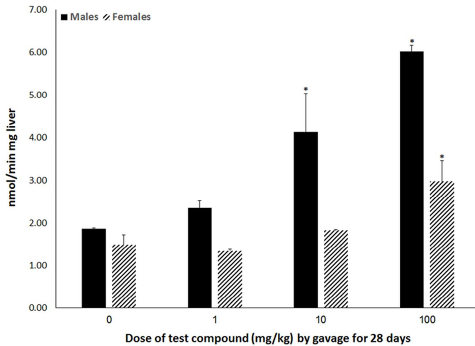
Figure 4. Hepatic peroxisome proliferation (mean \pm SD) of male or female C57Bl/6 mice given 2,3,3,3-tetrafluoro-2-(heptafluoropropoxy)-propanoate via gavage for 28 days. Acyl-CoA oxidase activity was measured in archived livers that had been collected from animals one day after exposure ended. *indicates a statistically significant increase in acyl-CoA oxidase activity relative to the 0 mg/kg group of the matching sex ( p < 0.05 ).
