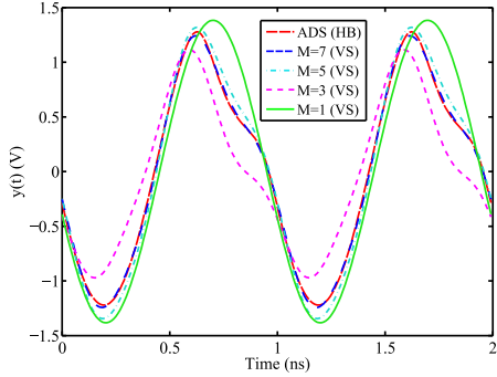
Fig. 11. Time domain output signals calculated based on the Volterra series (VS) model with different order and the ADS harmonic balance (HB) simulator with circuit model. The input signal is a single tone with frequency f = 1 GHz and power P_{in} = -0.5 dBm.
