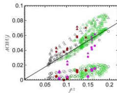
Figure 1. Ventilation plotted against square root of friction factor.
