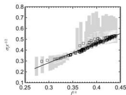
Figure 2. Vertical dispersion coefficient plotted against fourth root of friction factor.
