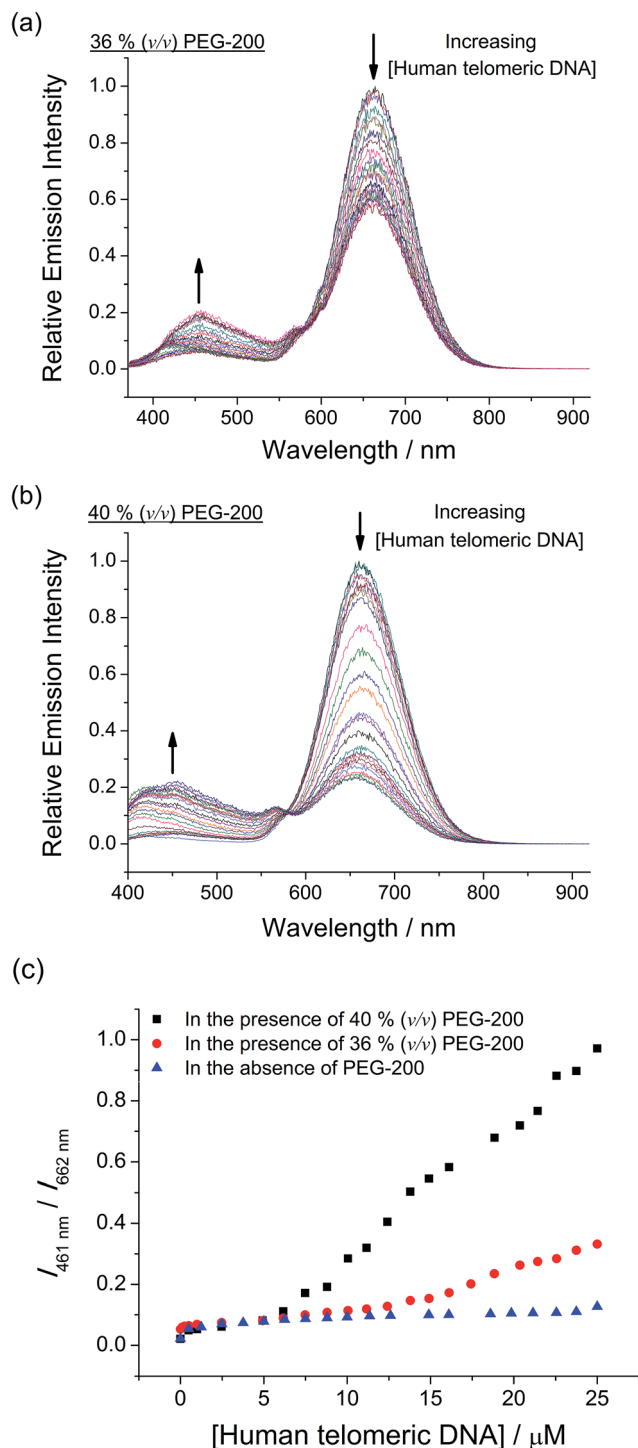
Fig. 7 Emission spectral changes of m PPE-Ala and 1 with increasing concentration of human telomeric DNA in the range of 0 to 25 \mu\text{M} in aqueous buffer solution (5 mM Tris-HCl, 50 mM KCl, pH 7.4) in the presence of (a) 36% (v/v) and (b) 40% (v/v) PEG-200. (c) Ratiometric emission of m PPE-Ala and 1 at 461 and 662 nm in aqueous buffer solution with different concentrations of human telomeric DNA in the range of 0 to 25 \mu\text{M} in the presence of 0% (v/v) ( \blacktriangle ), 36% (v/v) ( \bullet ) and 40% (v/v) ( \blacksquare ) PEG-200. Concentrations of m PPE-Ala and 1 were 50 \mu\text{M} and 20 \mu\text{M} respectively. Excitation was at 299 nm.
