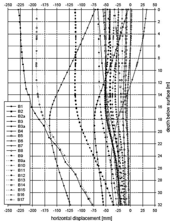
Figure 3. Wall deflection at final excavation stage (Schweiger 2002)
