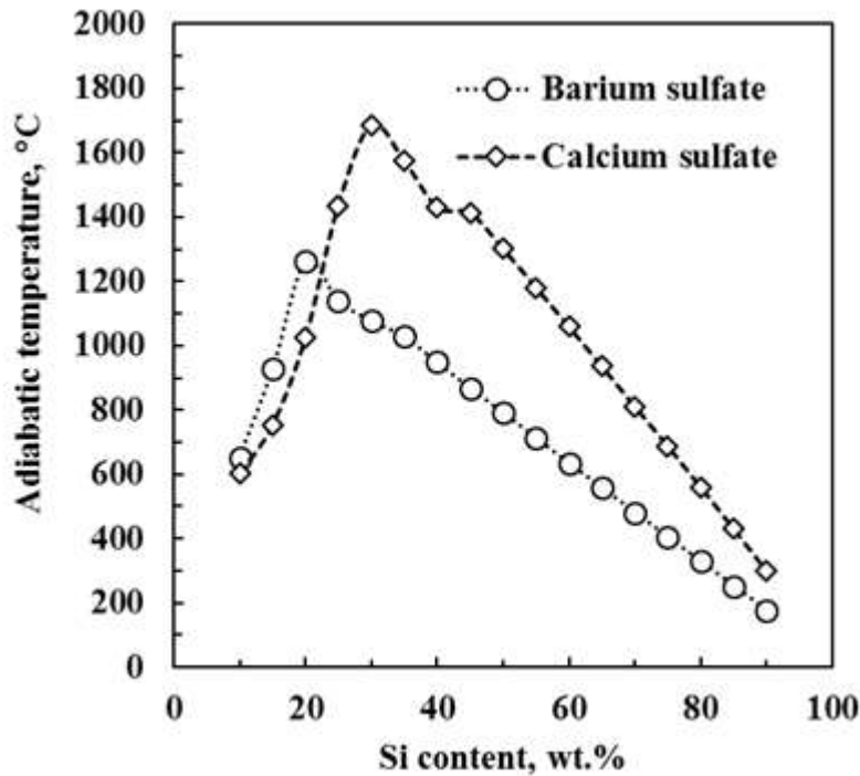
Figure 4. Comparison of the predicted adiabatic combustion temperature at different stoichiometries for both Si-CaSO 4 and Si-BaSO 4 systems using EKV1 software.
