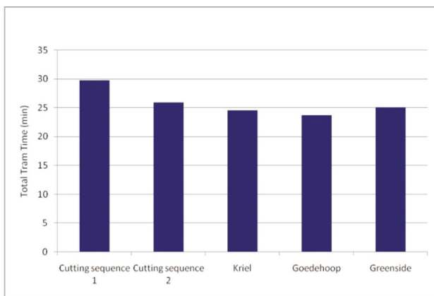
Figure 17 – Simulation results: comparison of the total trammung times of the simulated cutting sequences
