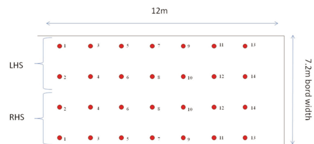
Figure 4 – Plan view of the ideal roofbolt installation sequence for a double-boom roofbolter (Van Staden, 2014)
