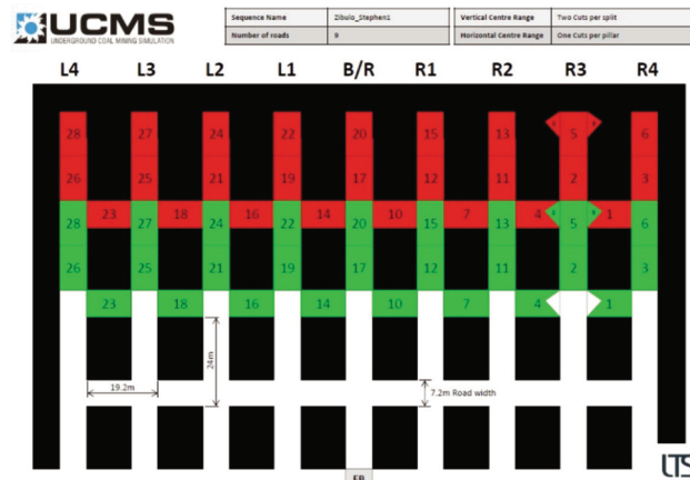
Figure 15 – Cutting sequence 1
