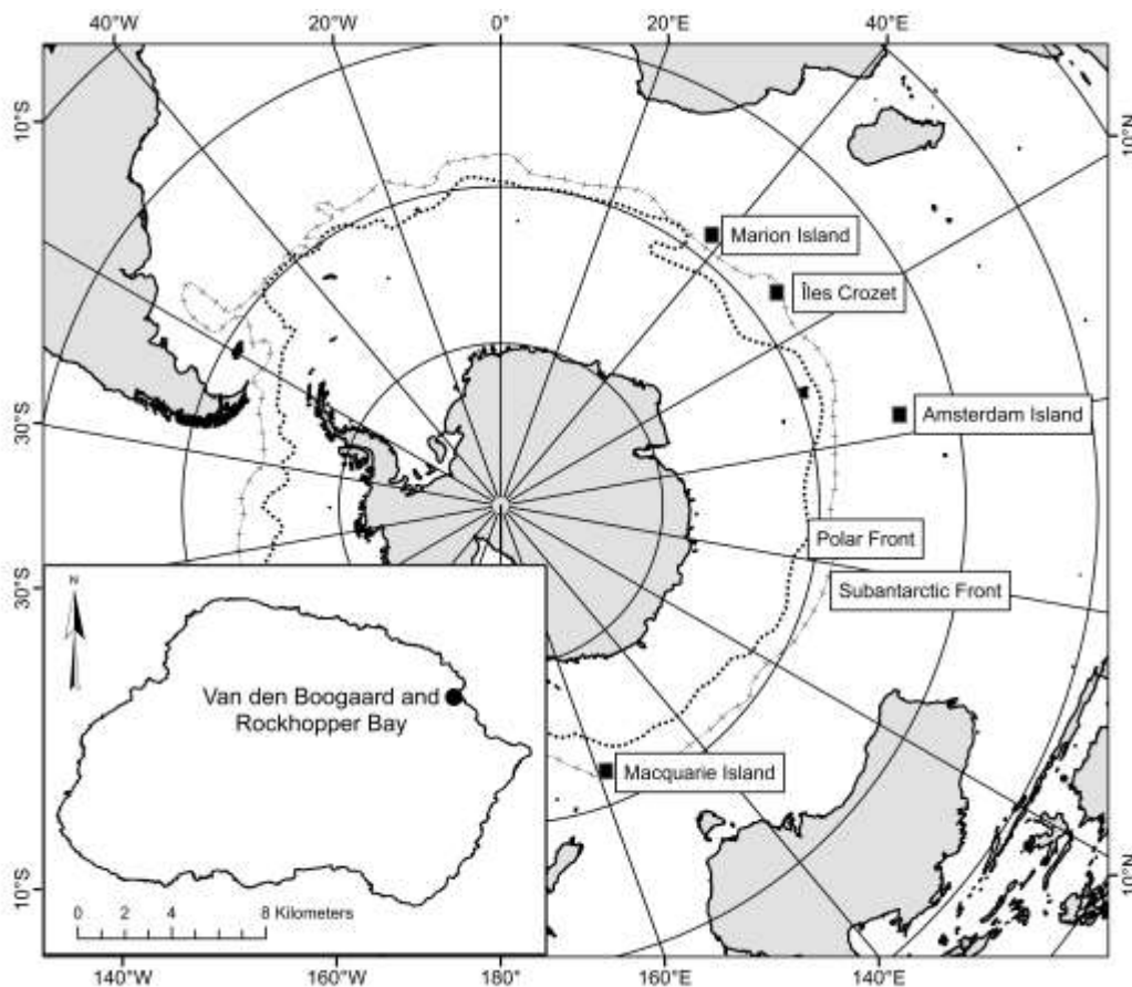
Figure 1: The position of Marion Island in the Southern Ocean in relation to Île de la Possession (Îles Crozet), Amsterdam Island and Macquarie Island as well as the Antarctic Polar Front, Subtropical Front and the Subantarctic Front. The location of Van den Boogaard and Rockhopper Bay beaches (study beaches) on Marion Island are indicated (inset).
