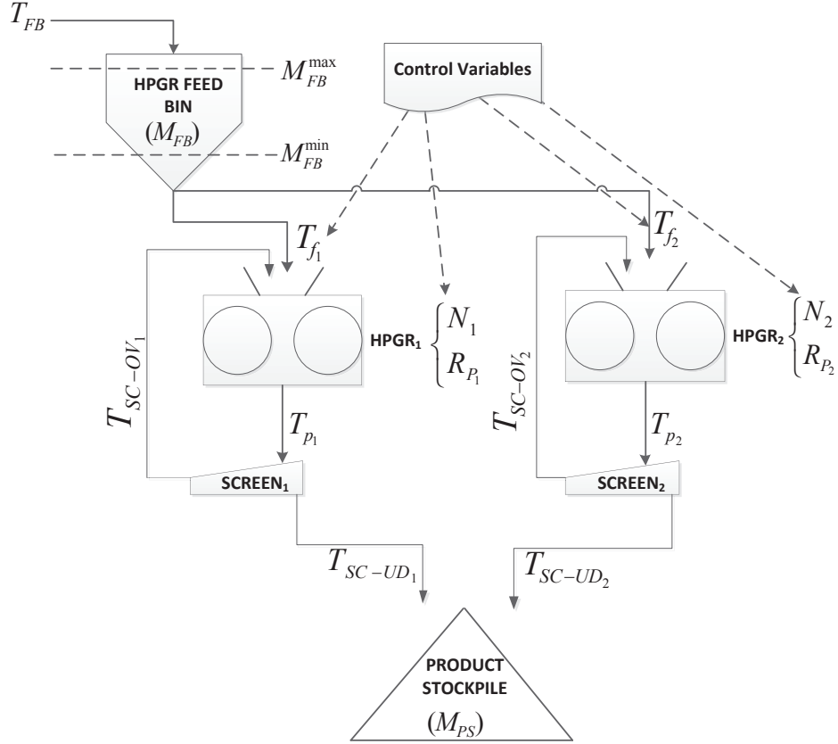
Figure 4: Schematic of a two parallel HPGR crushing circuit
