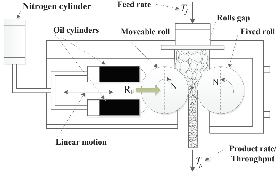
Figure 1: Cross-sectional representation of HPGR (adapted from [20])
