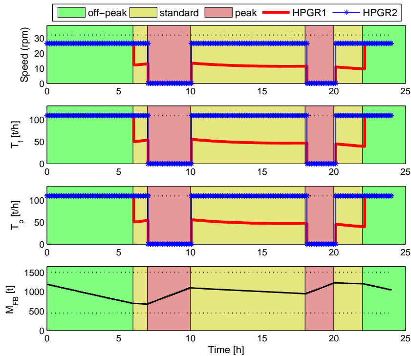
Figure 9: Systems optimization control technique with different overall drive efficiency, \eta_1 = 76\% , \eta_2 = 80.28\% using linprog function of Matlab Optimization Toolbox
