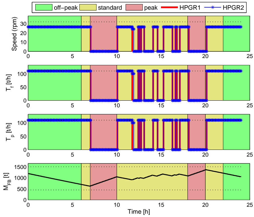
Figure 7: Systems optimization control technique with equal overall drive efficiency, \eta_1 = \eta_2 = 80.28\% using opti function of Opti Toolbox
