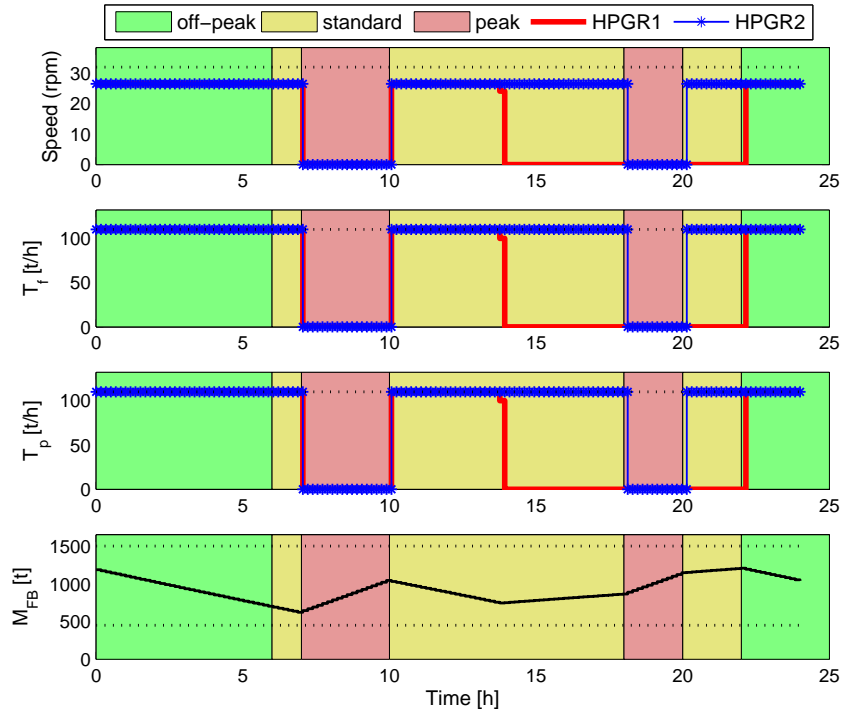
Figure 10: Systems optimization control technique with different overall drive efficiency, \eta_1 = 76\% , \eta_2 = 80.28\% using opti function of Opti Toolbox
