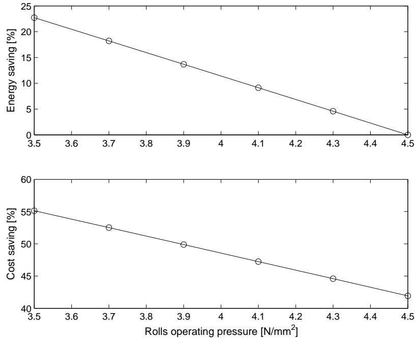
Figure 14: Sensitivity of rolls operating pressure on Energy and cost savings
