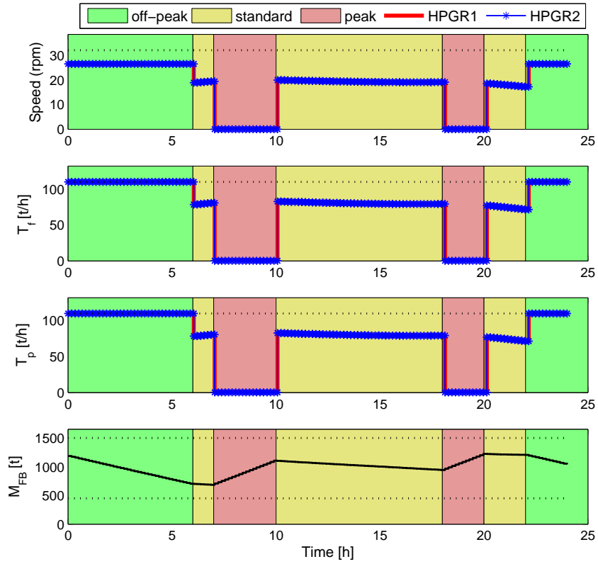
Figure 6: Systems optimization control technique with equal overall drive efficiency, \eta_1 = \eta_2 = 80.28\% using linprog function of Matlab Optimization Toolbox
