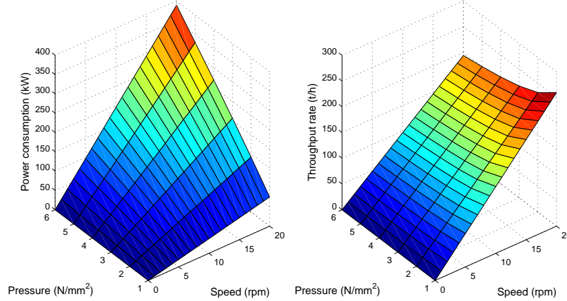
Figure 2: 3D plots of the analytical models of power consumption and throughput rate of HPGR machine
