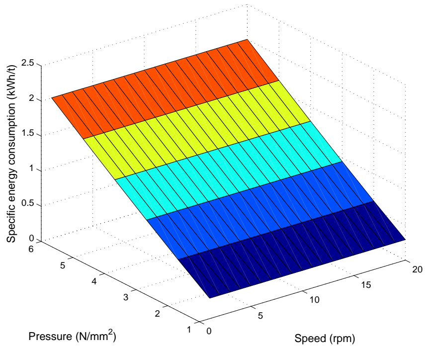
Figure 3: 3D plot of the analytical specific energy model of HPGR machine
