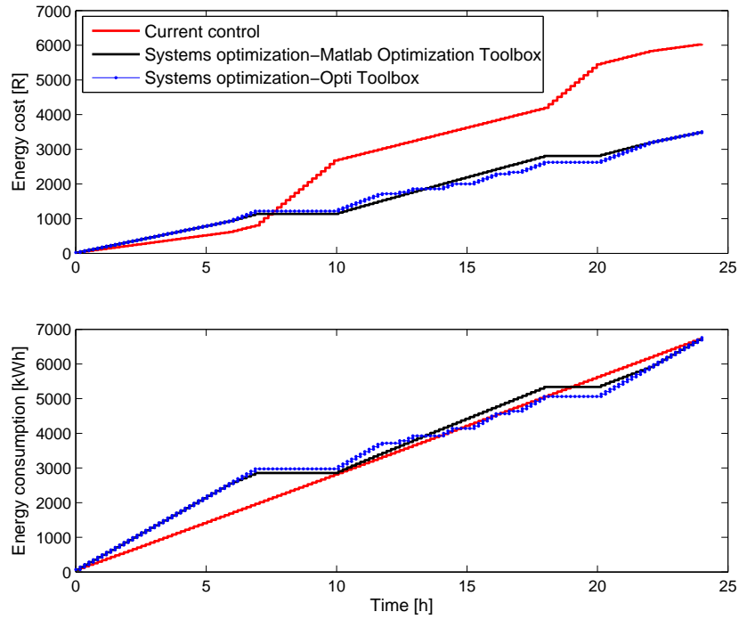
Figure 8: Cumulative energy cost and consumption with equal overall drive efficiency, \eta_1 = \eta_2 = 80.28\%
