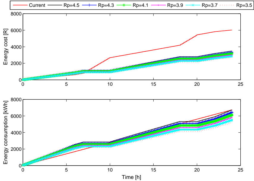
Figure 12: Sensitivity of rolls operating pressure on cumulative energy cost and energy consumption
