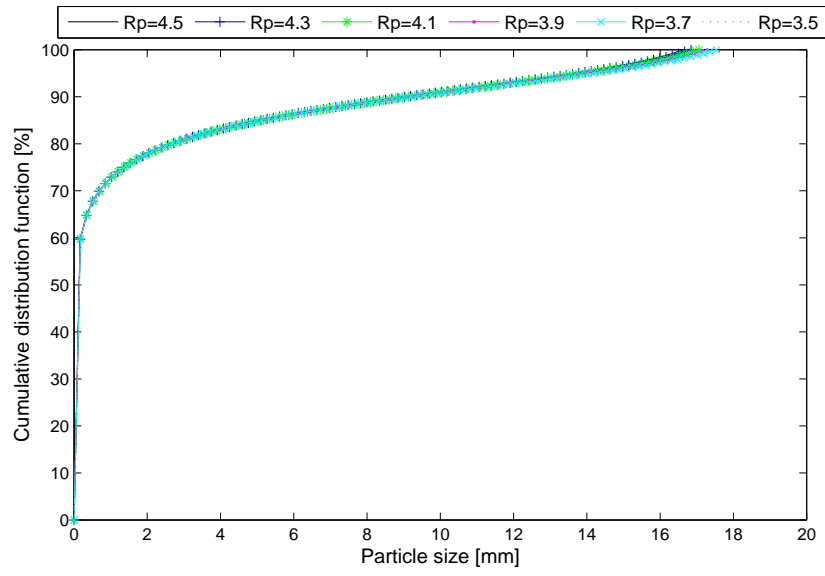
Figure 13: Sensitivity of rolls operating pressure on product size distribution
