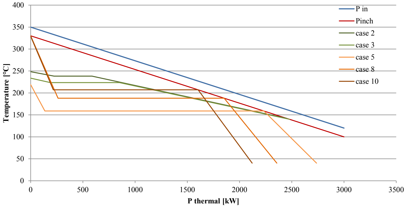
Figure 7 : Heating profile ORC and steam cycle
