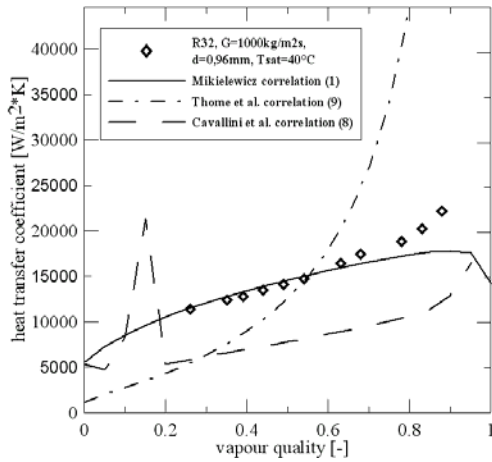
Figure 13. Comparison of heat transfer coefficient for R32 in relation to experimental data [6] using (1),(9),(8), d=0,96 \text{ mm} , G=1000 \text{ kg/m}^2\text{s} , T_{\text{sat}}=40^\circ\text{C}
