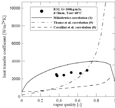
Figure 14. Comparison of heat transfer coefficient for R32 in relation to experimental data [4] using (1),(9),(8), d=8 \text{ mm} , G=100 \text{ kg/m}^2\text{s} , T_{\text{sat}}=40^\circ\text{C}
