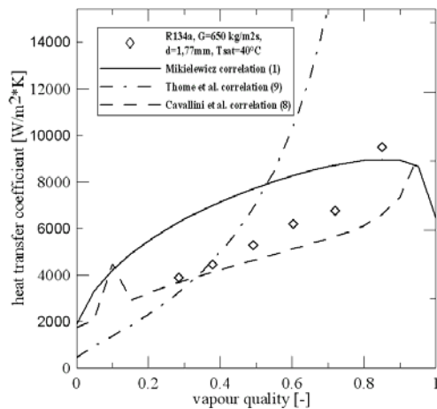
Figure 4. Comparison of heat transfer coefficient for R134a in relation to experimental data [5] using (1),(9),(8), d=1,77 mm, G=650\text{kg/m}^2\text{s} , T_{\text{sat}}=40^\circ\text{C}
