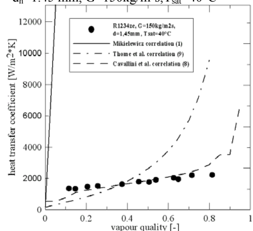
Figure 18. Comparison of heat transfer coefficient for R1234ze in relation to experimental data [9] using (1),(9),(8), d_h=1.45 \text{ mm} , G=150\text{kg/m}^2\text{s} , T_{\text{sat}}=40^\circ\text{C}
