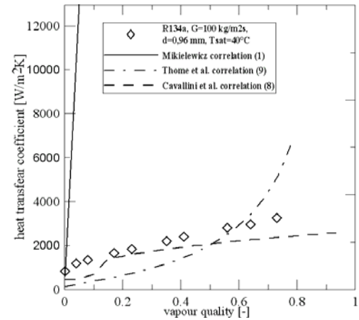
Figure 1. Comparison of heat transfer coefficient for R134a in relation to experimental data [6] using (1),(9),(8), d=0,96 mm, G=100 kg/m 2 s, T_{sat}=40^\circ\text{C}
