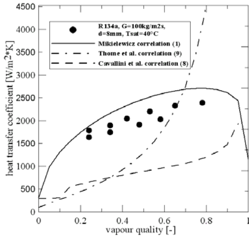
Figure 8. Comparison of heat transfer coefficient for R134a in relation to experimental data [4] using (1),(9),(8), d=8 mm, G=100 kg/m 2 s, T_{sat}=40^{\circ}\text{C}
