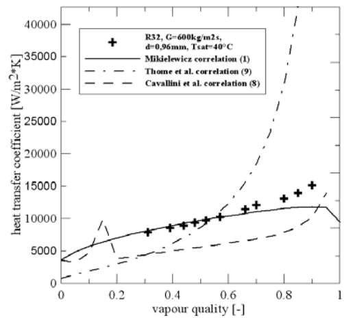
Figure 12. Comparison of heat transfer coefficient for R32 in relation to experimental data [6] using (1),(9),(8), d=0.96 mm, G=600 kg/m 2 s, T_{sat}=40^{\circ}\text{C}
