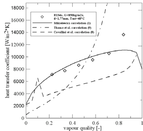
Figure 5. Comparison of heat transfer coefficient for R134a in relation to experimental data [5] using (1),(9),(9), d=1.77 mm, G=850\text{kg/m}^2\text{s} , T_{\text{sat}}=40^\circ\text{C}
