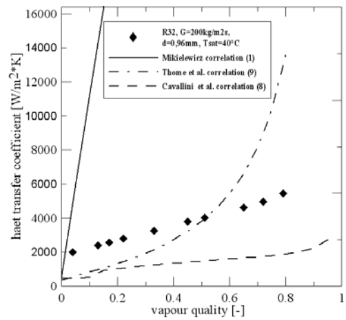
Figure 11. Comparison of heat transfer coefficient for R32 in relation to experimental data [6] using (1),(9),(8), d=0.96 mm, G=200 kg/m 2 s, T_{sat}=40^{\circ}\text{C}
