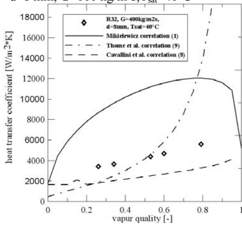
Figure 15 Comparison of heat transfer coefficient for R32 in relation to experimental data [4] using (1),(9),(8), d=8 \text{ mm} , G=400\text{kg/m}^2\text{s} , T_{\text{sat}}=40^\circ\text{C}
