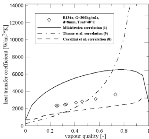
Figure 9. Comparison of heat transfer coefficient for R134a in relation to experimental data [4] using (1),(8),(9), d=8 mm, G=300 kg/m 2 s, T_{sat}=40^{\circ}\text{C}
