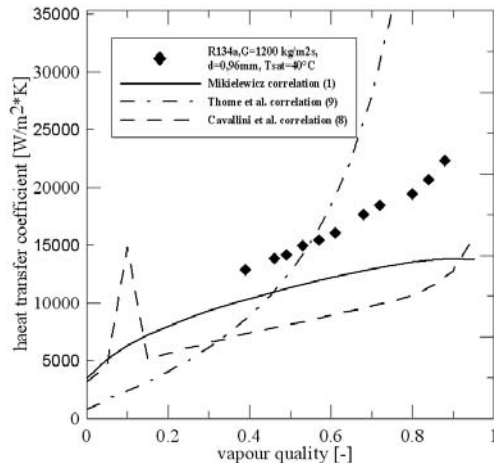
Figure 3. Comparison of heat transfer coefficient for R134a in relation to experimental data [6] using (1),(9),(8), d=0,96 mm, G=1200\text{kg/m}^2\text{s} , T_{\text{sat}}=40^\circ\text{C}
