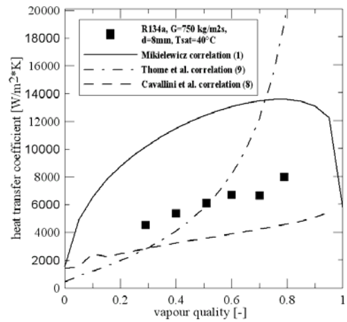
Figure 10. Comparison of heat transfer coefficient for R134a in relation to experimental data [4] using (1),(9),(8), d=8 mm, G=750 kg/m 2 s, T_{sat}=40^{\circ}\text{C}
