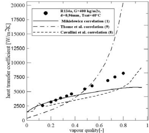
Figure 2. Comparison of heat transfer coefficient for R134a in relation to experimental data [6] using (1),(9),(8), d=0,96 mm, G=400 kg/m 2 s, T_{sat}=40^\circ\text{C}
