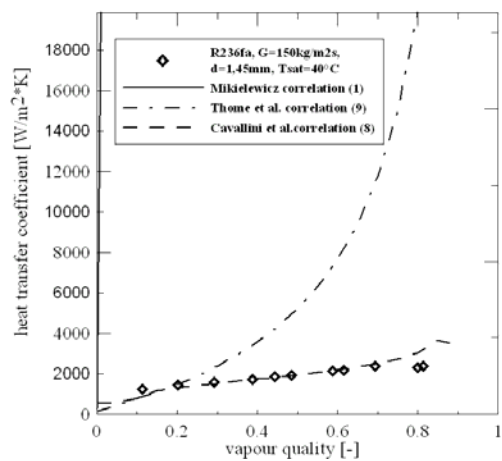
Figure 17. Comparison of heat transfer coefficient for R236fa in relation to experimental data [9] using (1),(9),(8), d_h=1.45 \text{ mm} , G=150\text{kg/m}^2\text{s} , T_{\text{sat}}=40^\circ\text{C}
