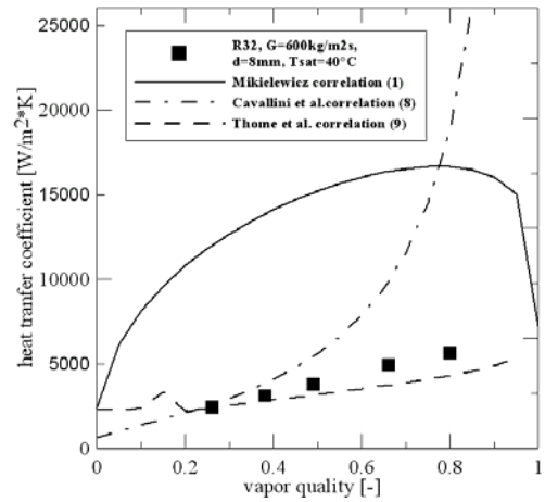
Figure 16. Comparison of heat transfer coefficient for R32 in relation to experimental data [4] using (1),(9),(8), d=8 \text{ mm} , G=600\text{kg/m}^2\text{s} , T_{\text{sat}}=40^\circ\text{C}
