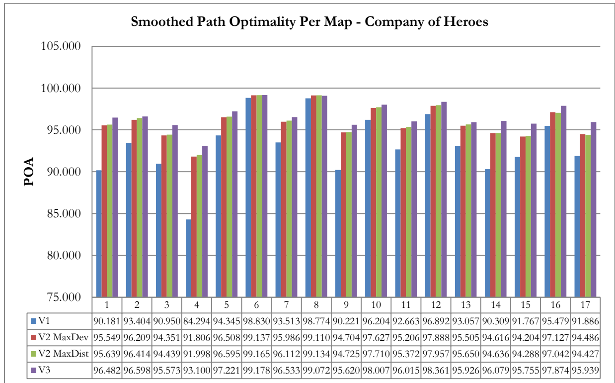
Figure 8.23: Per-map SGA* path optimality measurements for the "Company of Heroes" test set
