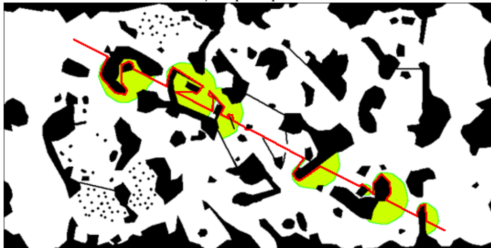
b) SGA* variant 1 unsmoothed path
