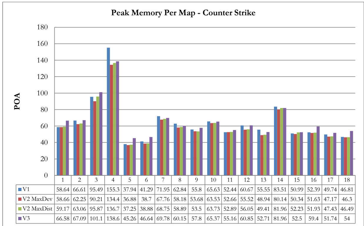
Figure 8.16: Per-map SGA* performance results for the "Counter-Strike" test set
