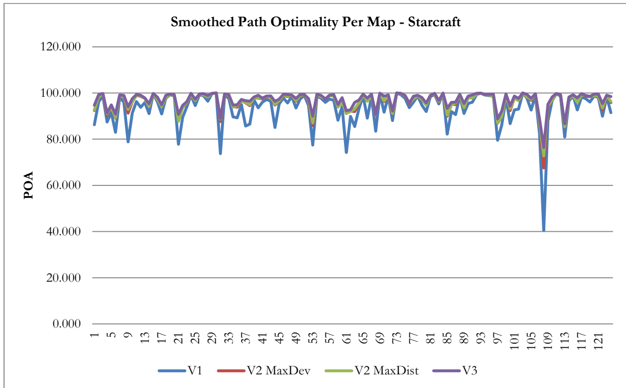
Figure 8.36: Per-map SGA* path optimality measurements for the "Starcraft" test set
