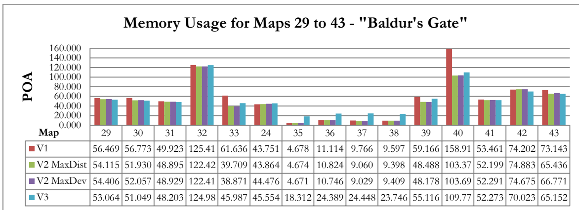
Figure 8.28: Per-map SGA* performance results for maps 29-43 of the “Baldur’s Gate” test set
