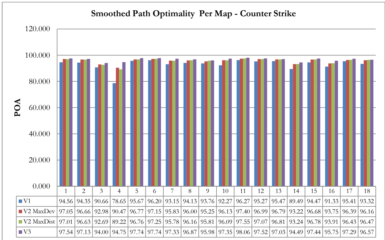
Figure 8.18: Per-map SGA* path optimality measurements for the "Counter-Strike" test set
