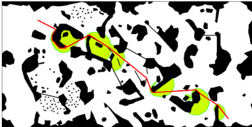
c) SGA* variant 1 smoothed path
