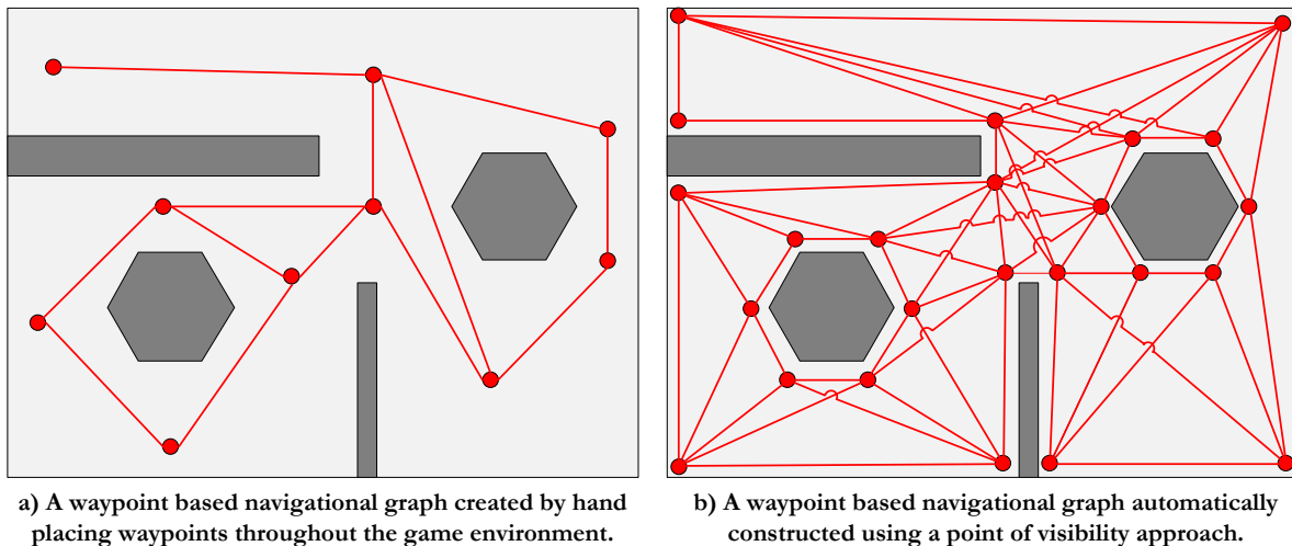
Figure 3.1: Waypoint based navigational graphs
