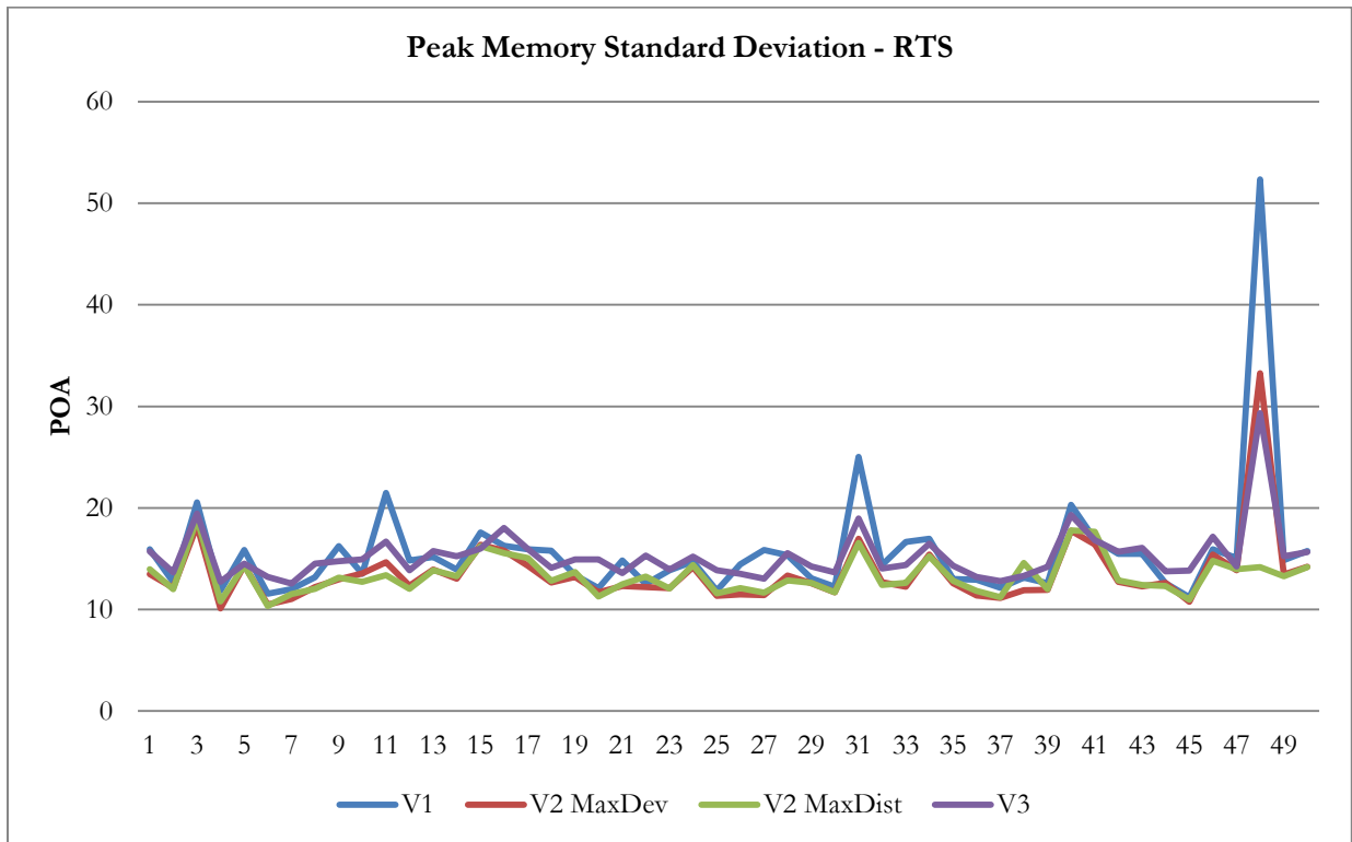
Figure 8.42: The standard deviations for search times and peak memory usage for the "Pseudo RTS" test set
