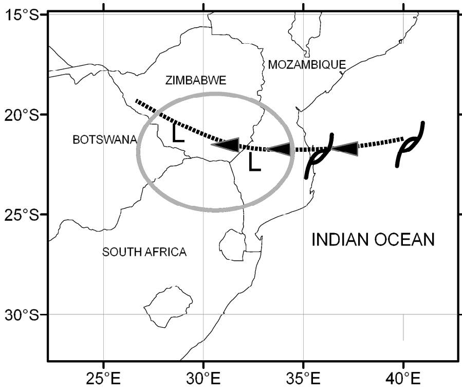
Figure 2 A track followed by several tropical systems from the SWIO making landfall and moving westward over southern Africa.
