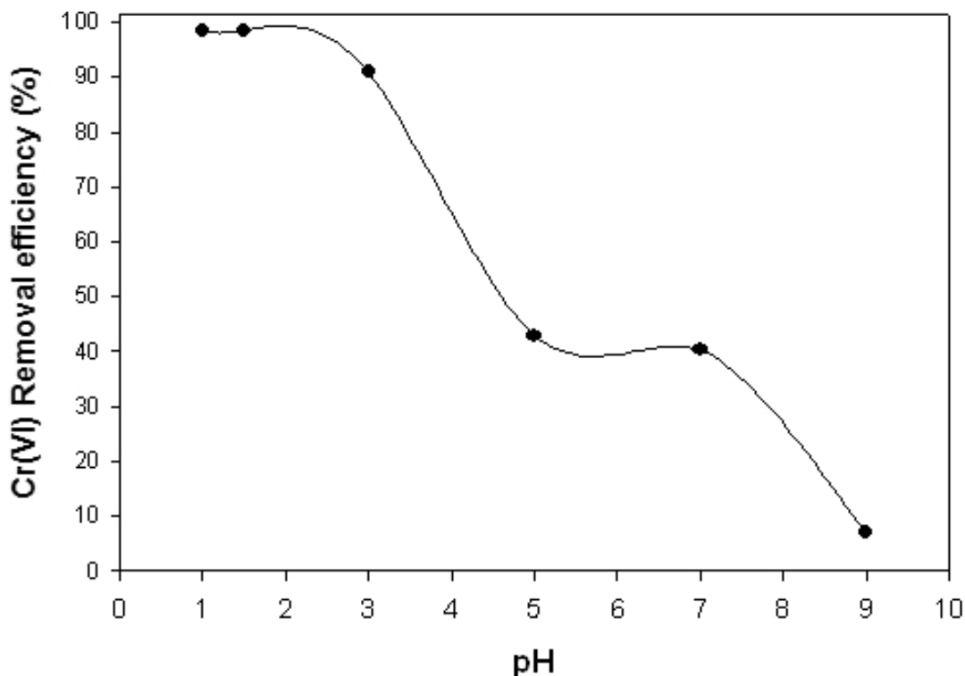
Fig. 3. Effect of pH on Cr(VI) removal efficiency (adsorbent dosage 10 g L -1 and contact time of 120 min).
