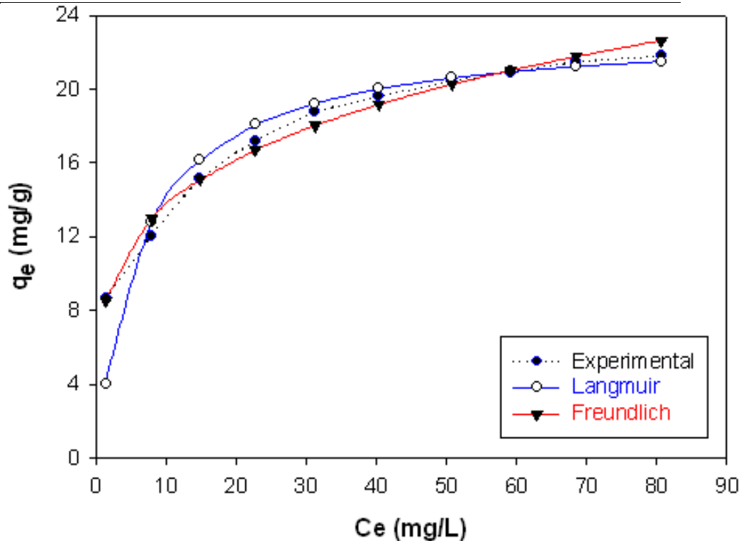
Fig. 5. Non-linear isotherm plots for Cr(VI) adsorption onto vermiculite (pH 1.5; adsorbent dosage 10 \text{ g L}^{-1} and contact time 120 min).
