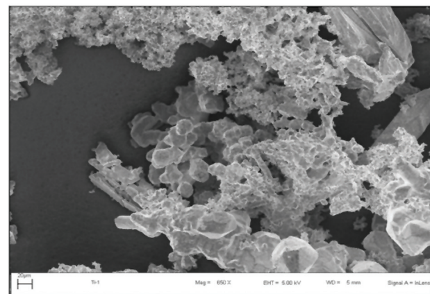
Figure 13—SEM of product (scale = 20 \mu\text{m} )
