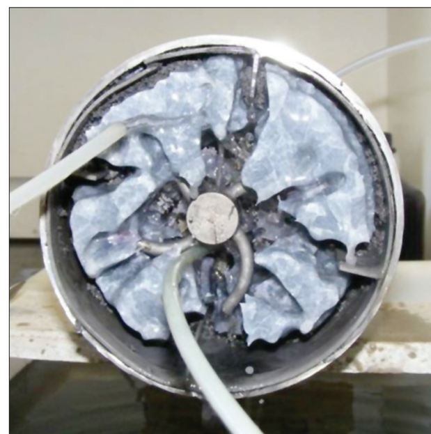
Figure 3—Leaching of reactor contents
