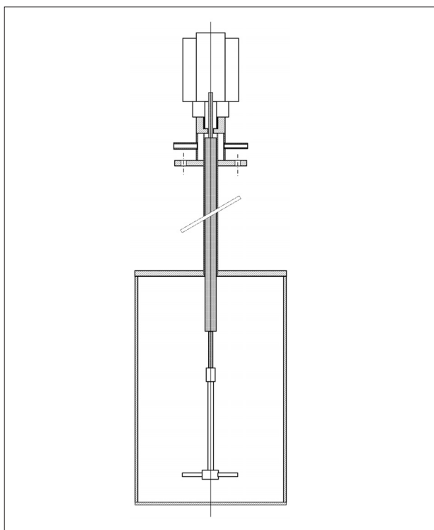
Figure 1—Drawing of the reactor
