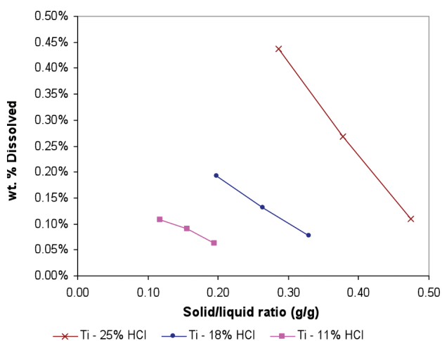
Figure 3—Effect of solid/liquid mass ratio on titanium dissolution (90°C, d_{50} = 185 \mu\text{m} , 100 rpm)
