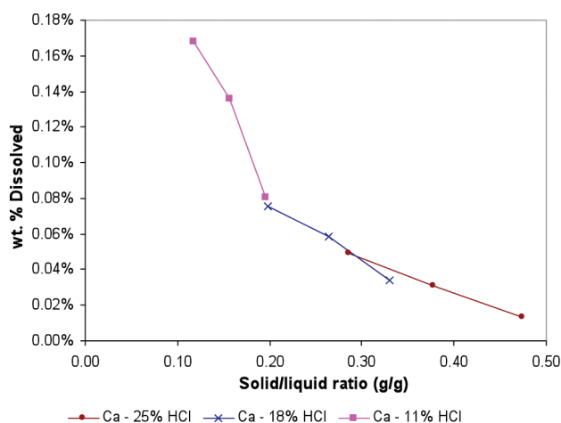
Figure 2—Effect of solid/liquid mass ratio on calcium dissolution (90°C, d_{50} = 185 \mu\text{m} , 100 rpm)
