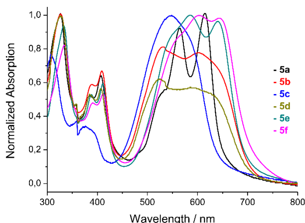
Figure 2. Normalized UV-Vis absorption of compounds for compounds 5a (a), 5b (b), 5c (c), 5d (d), 5e (e) and 5f (f) as thin-film, spin-coated from chloroform solution (10 mg/mL, 1000 rpm/60 s).
