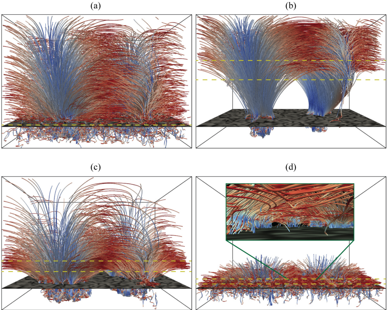
Figure 1. : Magnetic configuration in the Bifrost simulation in perspective view. The volume measures 24 \times 24 \text{ Mm}^2 horizontally, 14 Mm vertically. The visible surface (optical depth unity at 500 nm) is specified with a synthetic continuum image. The plotted field lines start at locations that are randomly distributed through a thin layer at a selected height and then traced upward and downward to chart fields elsewhere (a) throughout the entire simulation volume (starting points of the tracing located in a 0–100 km layer), (b) only those that reach the lower corona (starting points between 5000 and 7000 km), (c) adding those that reach the upper chromosphere and transition region (starting points 1800–2800 km), (d) adding those that reach the lower chromosphere traced from starting points at 500–1000 km and with a cut at 1400 km height for better visibility. The colors represent inclination, from vertical (blue) to horizontal (red). A small 700-km high cutout of the region between the two main footpoints is magnified in the inset in (d).
