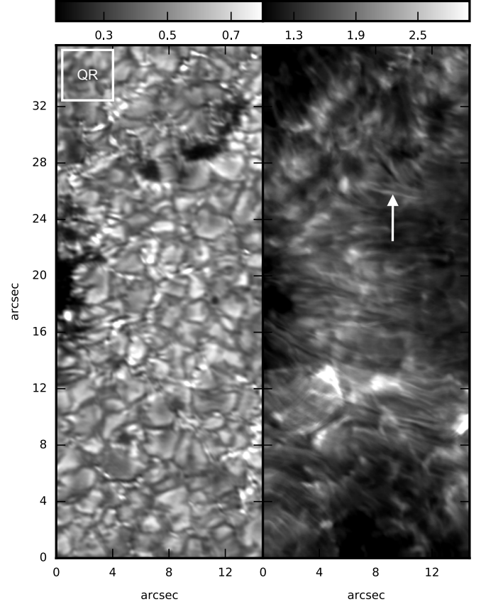
Figure 1. : Right: Example of a Ca II H image recorded by SUNRISE/SUFI. Left: An image recorded at 300 nm, aligned with the Ca II H filtergram. The white arrow in the right panel indicates a sample slender Ca II H fibril (SCF). The white box marks the quiet region (QR) used to normalize the intensities in the Ca II H and 300 nm images.
