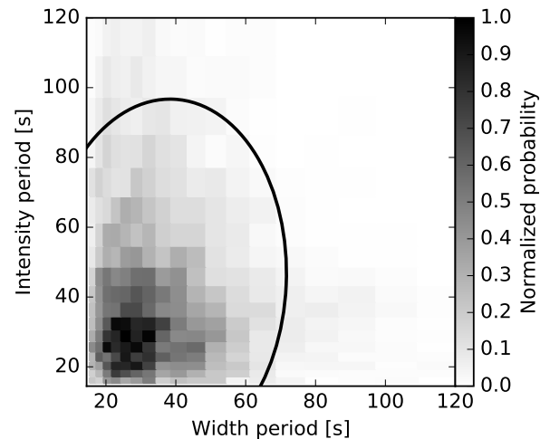
Figure 5. : Two-dimensional histogram showing the relation between the periods of the width and the intensity oscillations in SCFs. The bin size follows the period resolution that is limited by the life time of the fibrils. The black curved line indicates the 95% confidence level.
