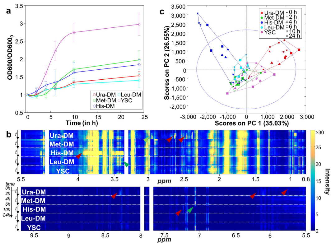
Figure 1. Yeast growth. (a) Graphic representation of cell growth at the different media (normalized for the initial OD 600 ). (b) Heatmap representation of the 1 H NMR spectra for the five different time-courses. Each row corresponds to the average of 3 spectra. Within each time-course studied, data are presented row-wise following an increasing time order. The red and green arrows point to peak signals of some metabolites accumulated (increasing intensity) or consumed (decreasing intensity) over time. (c) PCA scores projection of the mean-centered spectral dataset on PC1 and PC2 subspace. DM, Drop-out Media; YSC, Yeast Nitrogen Base Synthetic Complete medium.
