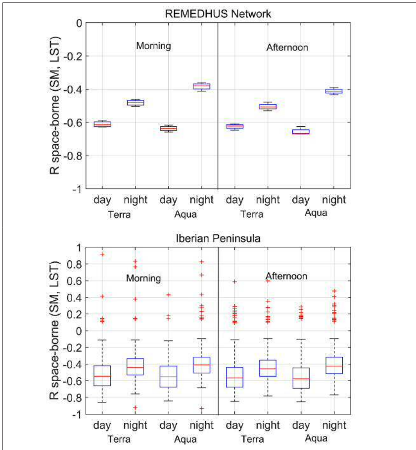
Figure 2 - Correlation (R) of space-borne SMOS SM at morning and afternoon passes and MODIS LST Terra day, Terra night, Aqua day, and Aqua night over the REMEDHUS region (top) and the Iberian Peninsula (bottom).
