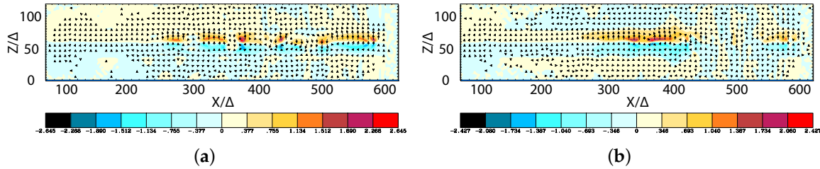
Figure 4. Isocontour plots of the azimuthal component of magnetic field B_y intensity at the center of the jets for (a) e^-p^+ and (b) e^\pm jets ( y/\Delta = 63 ) at time t = 500 \omega_{pe}^{-1} . The disruption of helical magnetic fields is caused by instabilities and/or reconnection.
