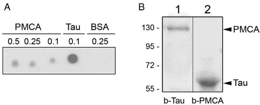
Fig. 5. Tau and PMCA interaction. (A) Dot blot assay: pig brain purified PMCA, recombinant tau and BSA were applied onto a nitrocellulose membrane at the indicated amounts ( \mu\text{g} ). After blocking and washing, the membrane was incubated for 2 h at 37 °C with 0.18 \mu\text{g} of tau, followed by several washes to remove unbound tau and overnight incubation at 4 °C with Tau5 antibody (1:1000), which binds to total tau. The presence of bound tau was detected by chemiluminescence. (B) Five \mu\text{g} of pig brain PMCA (lane 1) or 2.5 \mu\text{g} of recombinant tau (lane 2) were subjected to 10% SDS-PAGE and subsequently transferred onto nitrocellulose membranes and incubated with biotinylated-tau (b-Tau) or biotinylated-PMCA (b-PMCA) as indicated in Methods (lanes 1 and 2, respectively). After washing away unbound protein, membranes were incubated with ExtrAvidin-Peroxidase and binding was detected by chemiluminescence.
