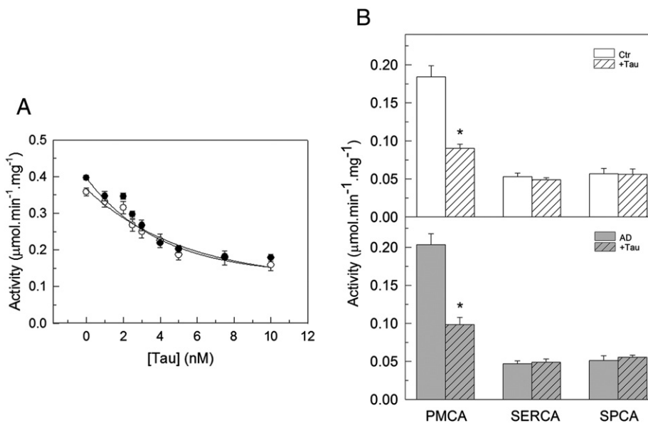
Fig. 2. Effect of tau on Ca 2+ -ATPase activity in membrane vesicles from Alzheimer's disease (AD) and age-matched control (Ctr) human brain tissues. A) The total Ca 2+ -ATPase activity was measured in 20 μg of MV from Ctr (○) and AD (●) brain, as described in Methods, in the presence of the indicated concentrations of tau. B) Specific PMCA, SERCA and SPCA activities were assayed in 20 μg of MV from Ctr (white bars) and AD (grey bars) human brain in the absence (empty bars) and presence (dashed bars) of 7.5 nM tau. Data are mean ± SE values obtained from 6 experiments performed in membrane fractions obtained from AD cases (n = 7) and age-matched controls (n = 6).
