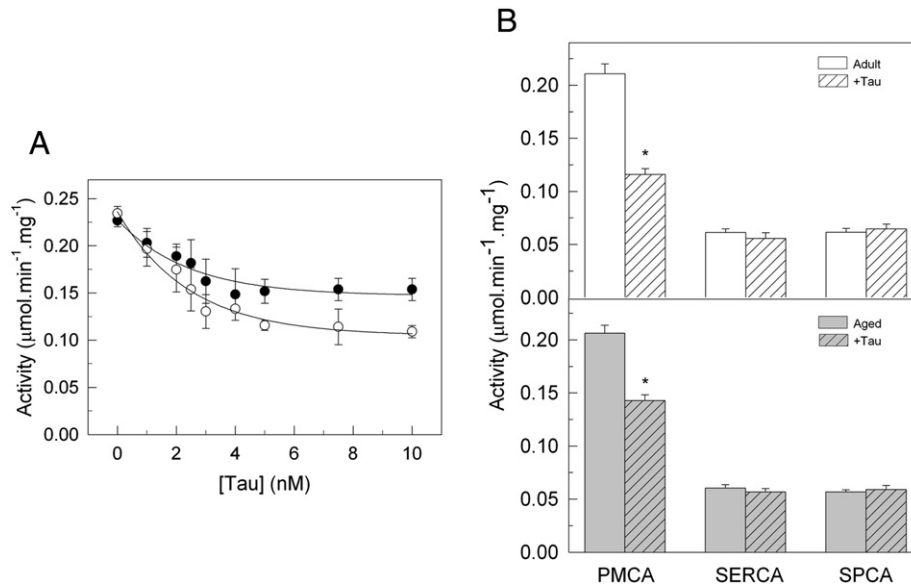
Fig. 1. Effect of tau on Ca 2+ -ATPase activity in membrane vesicles of adult and aged mice brain. A) The total Ca 2+ -ATPase activity was measured in 10 μg of MV from adult (○) and aged (●) mice brain as described in Methods, in the presence of the indicated concentrations of tau. B) The total Ca 2+ -ATPase activity and specific PMCA, SERCA and SPCA activities were assayed in 10 μg of MV from adult (white bars) and aged (grey bars) mice brain in the absence (empty bars) and presence (dashed bars) of 7.5 nM tau. Data are mean ± SE values obtained from 6 experiments performed in 3 adult and 3 aged mice preparations.
